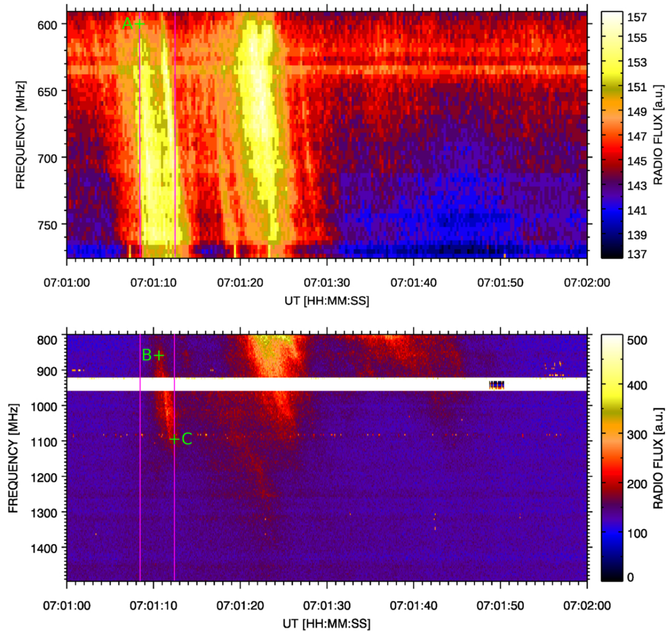
Figure 1. from Mehdi Yousefzadeh et al 2026 Astrophys. J. 1007 doi:10.3847/1538-4357/ae8771 https://dx.doi.org/10.3847/1538-4357/ae8771 © 2026. The Author(s). Published by the American Astronomical Society.
