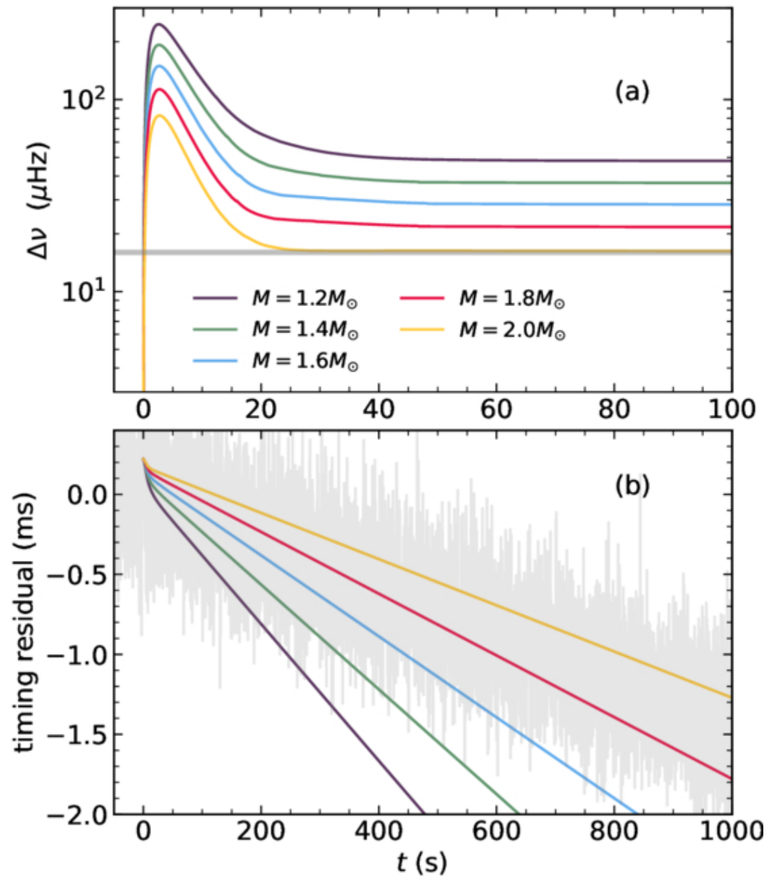
Figure 8. from Zhonghao Tu and Ang Li 2026 Astrophys. J. 1007 doi:10.3847/1538-4357/ae8768 https://dx.doi.org/10.3847/1538-4357/ae8768 © 2026. The Author(s). Published by the American Astronomical Society.
