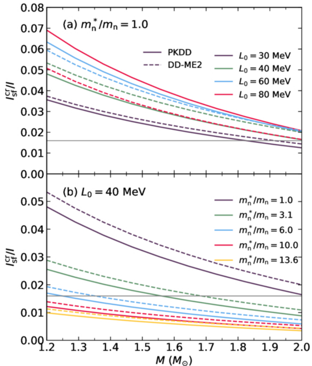
Figure 5. from Zhonghao Tu and Ang Li 2026 Astrophys. J. 1007 doi:10.3847/1538-4357/ae8768 https://dx.doi.org/10.3847/1538-4357/ae8768 © 2026. The Author(s). Published by the American Astronomical Society.
