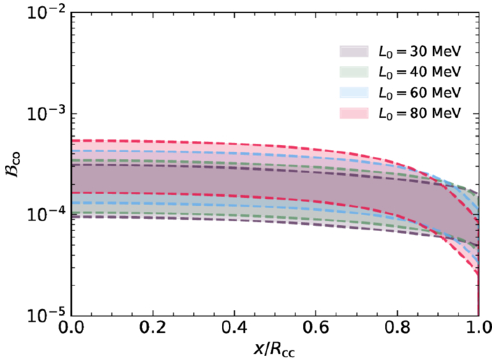
Figure 2. from Zhonghao Tu and Ang Li 2026 Astrophys. J. 1007 doi:10.3847/1538-4357/ae8768 https://dx.doi.org/10.3847/1538-4357/ae8768 © 2026. The Author(s). Published by the American Astronomical Society.
