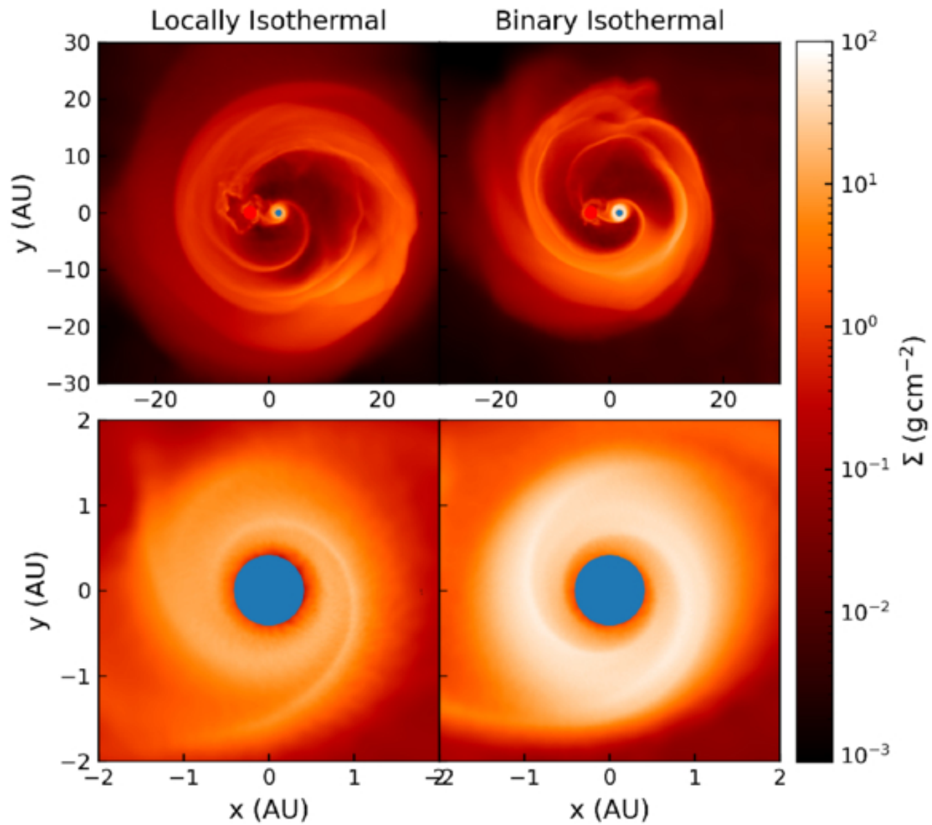
Figure 6. from Shunquan Huang et al 2026 Astrophys. J. 1006 doi:10.3847/1538-4357/ae875d https://dx.doi.org/10.3847/1538-4357/ae875d © 2026. The Author(s). Published by the American Astronomical Society.
