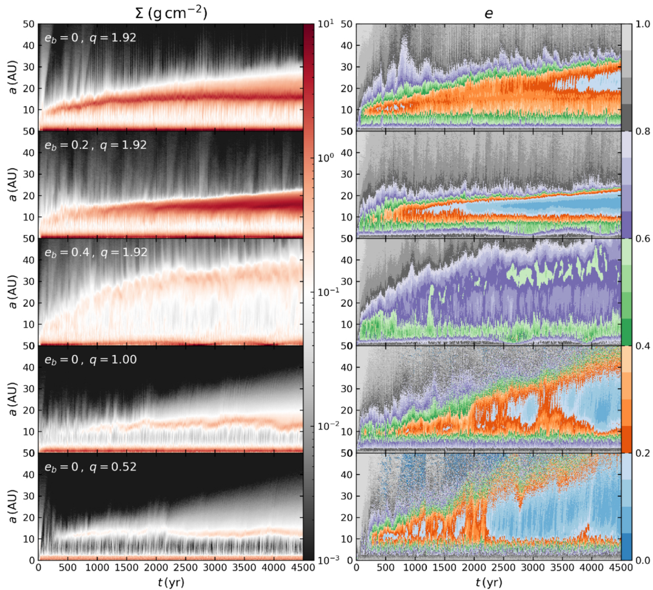
Figure 5. from Shunquan Huang et al 2026 Astrophys. J. 1006 doi:10.3847/1538-4357/ae875d https://dx.doi.org/10.3847/1538-4357/ae875d © 2026. The Author(s). Published by the American Astronomical Society.
