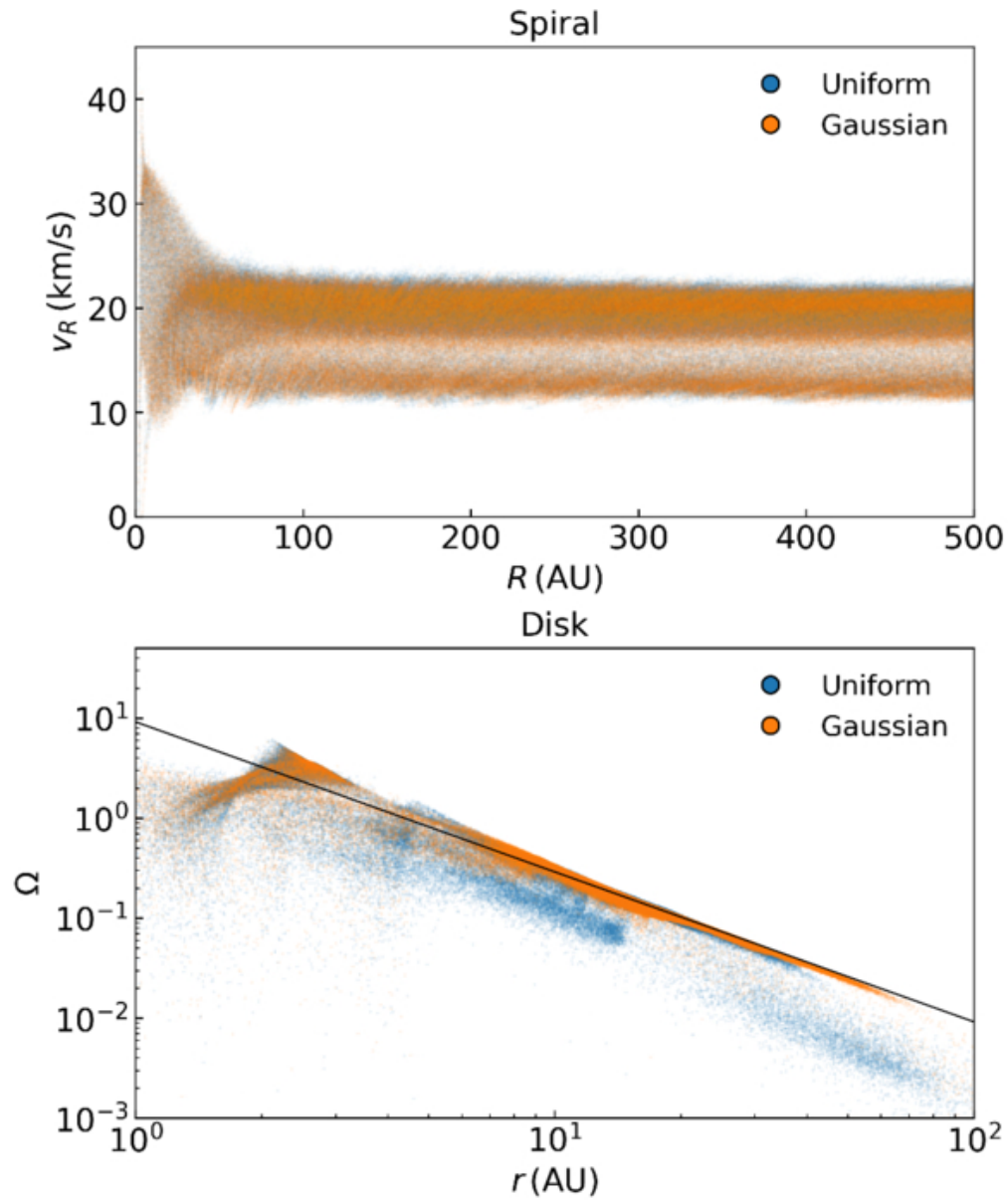
Figure 3. from Shunquan Huang et al 2026 Astrophys. J. 1006 doi:10.3847/1538-4357/ae875d https://dx.doi.org/10.3847/1538-4357/ae875d © 2026. The Author(s). Published by the American Astronomical Society.
