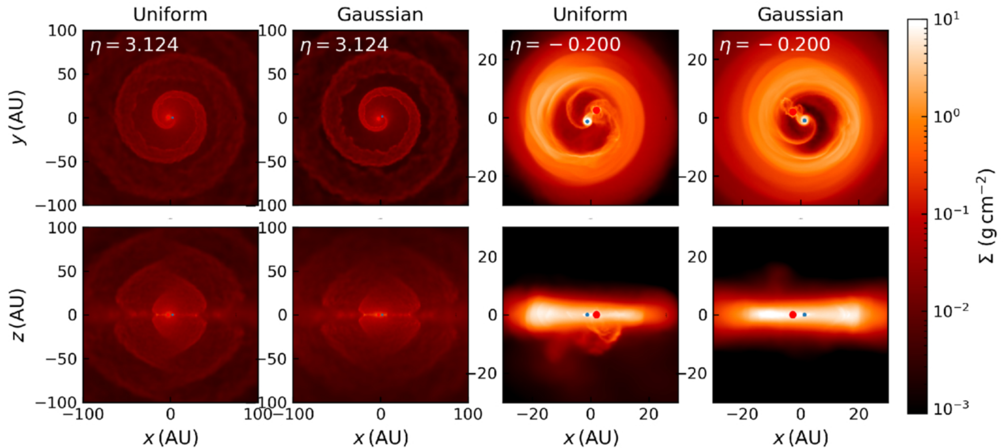
Figure 2. from Shunquan Huang et al 2026 Astrophys. J. 1006 doi:10.3847/1538-4357/ae875d https://dx.doi.org/10.3847/1538-4357/ae875d © 2026. The Author(s). Published by the American Astronomical Society.
