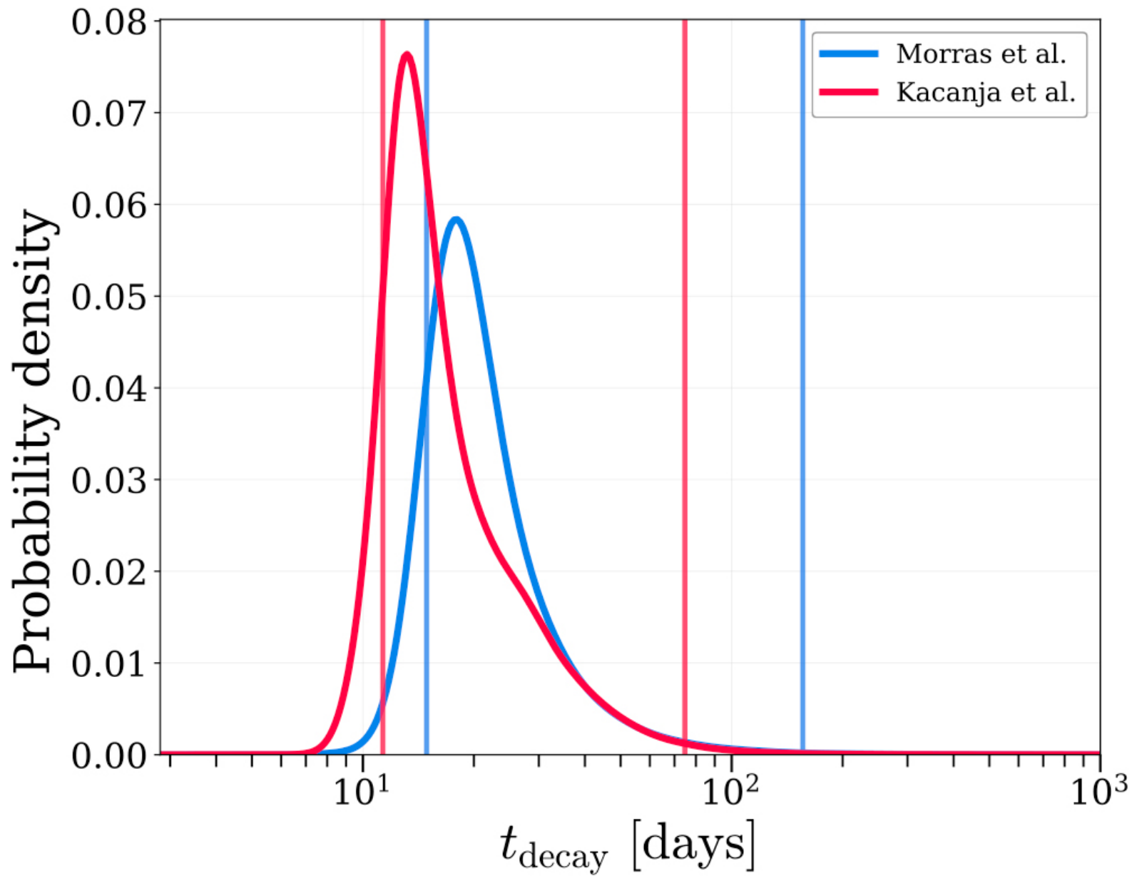
Figure 5. from A. Vincent Paul et al 2026 Astrophys. J. 1006 doi:10.3847/1538-4357/ae8759 https://dx.doi.org/10.3847/1538-4357/ae8759 © 2026. The Author(s). Published by the American Astronomical Society.
