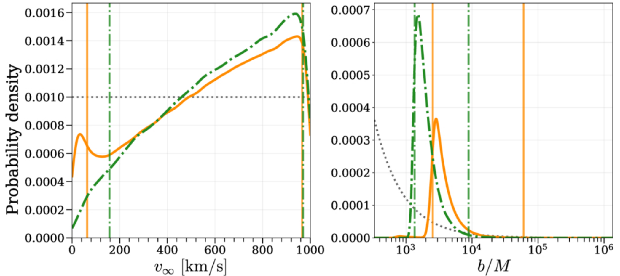
Figure 3. from A. Vincent Paul et al 2026 Astrophys. J. 1006 doi:10.3847/1538-4357/ae8759 https://dx.doi.org/10.3847/1538-4357/ae8759 © 2026. The Author(s). Published by the American Astronomical Society.
