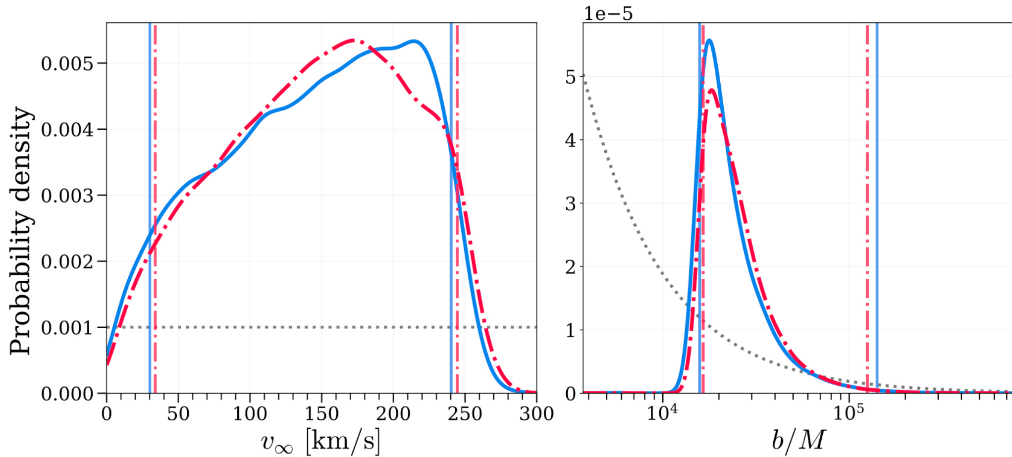
Figure 1. from A. Vincent Paul et al 2026 Astrophys. J. 1006 doi:10.3847/1538-4357/ae8759 https://dx.doi.org/10.3847/1538-4357/ae8759 © 2026. The Author(s). Published by the American Astronomical Society.
