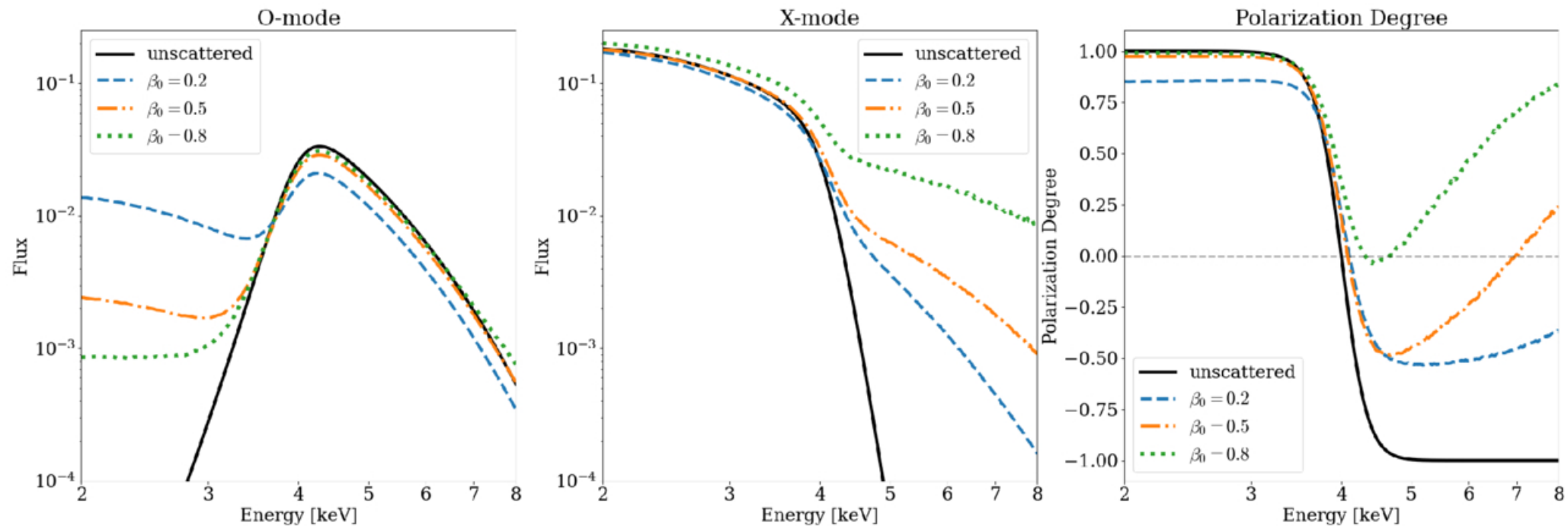
Figure 7. from Tu Guo and Dong Lai 2026 Astrophys. J. 1007 doi:10.3847/1538-4357/ae8758 https://dx.doi.org/10.3847/1538-4357/ae8758 © 2026. The Author(s). Published by the American Astronomical Society.
