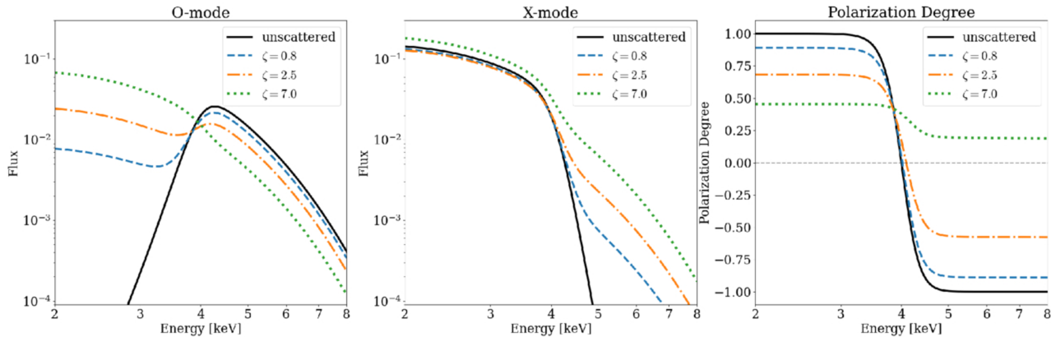
Figure 2. from Tu Guo and Dong Lai 2026 Astrophys. J. 1007 doi:10.3847/1538-4357/ae8758 https://dx.doi.org/10.3847/1538-4357/ae8758 © 2026. The Author(s). Published by the American Astronomical Society.
