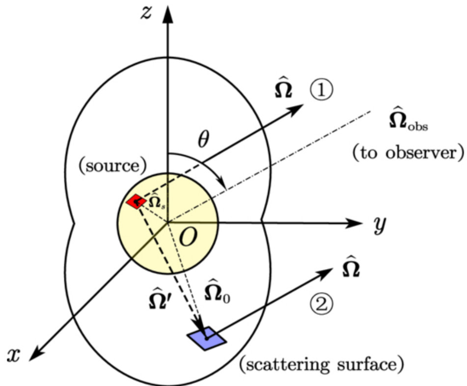
Figure 1. from Tu Guo and Dong Lai 2026 Astrophys. J. 1007 doi:10.3847/1538-4357/ae8758 https://dx.doi.org/10.3847/1538-4357/ae8758 © 2026. The Author(s). Published by the American Astronomical Society.
