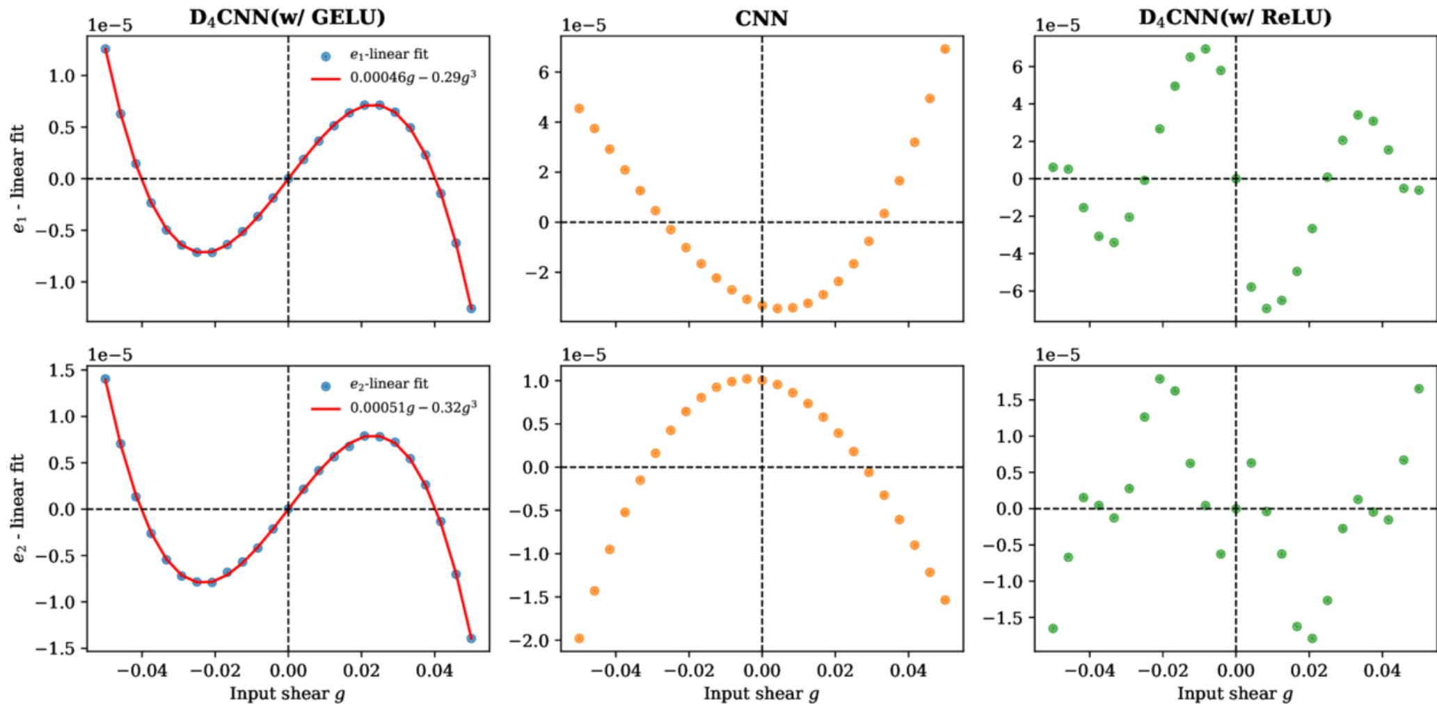
Figure 8. from Shurui Lin et al 2026 Astrophys. J. 1006 doi:10.3847/1538-4357/ae84b2 https://dx.doi.org/10.3847/1538-4357/ae84b2 © 2026. The Author(s). Published by the American Astronomical Society.
