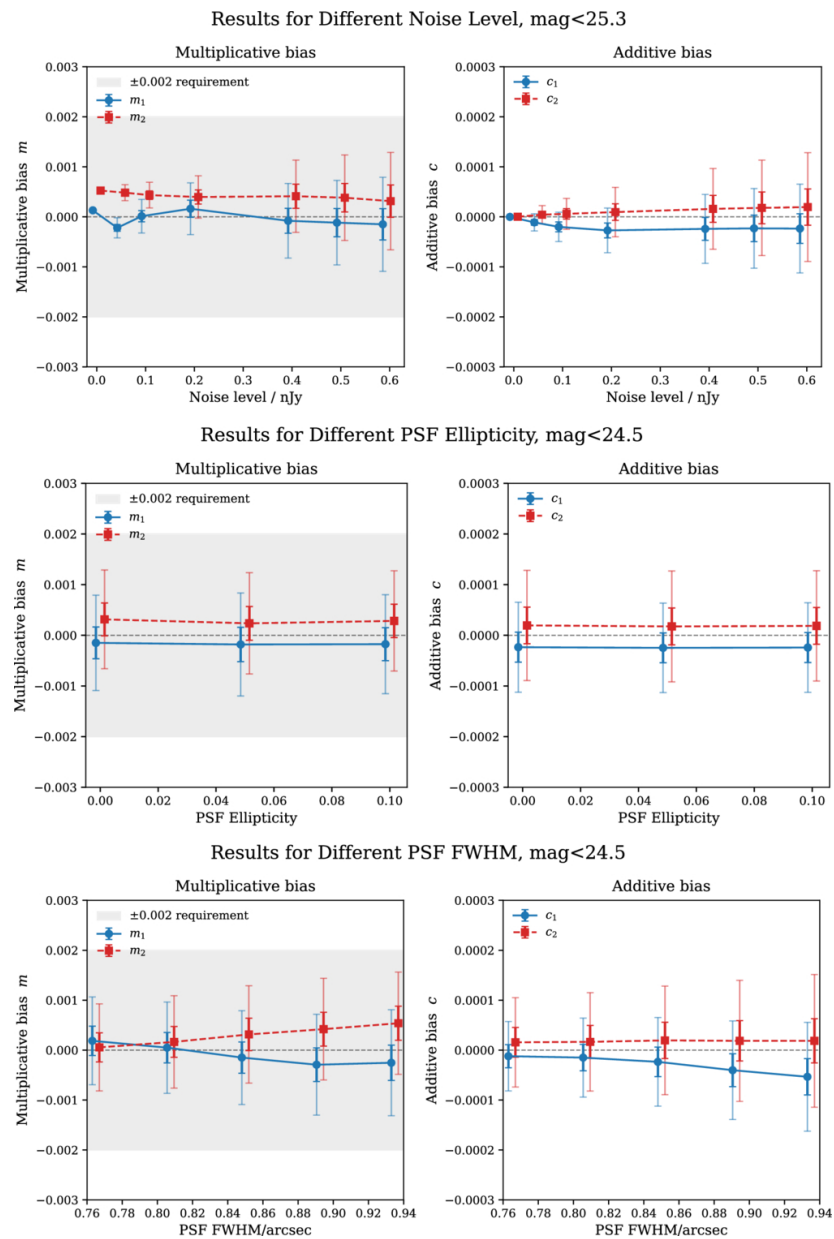
Figure 4. from Shurui Lin et al 2026 Astrophys. J. 1006 doi:10.3847/1538-4357/ae84b2 https://dx.doi.org/10.3847/1538-4357/ae84b2 © 2026. The Author(s). Published by the American Astronomical Society.
