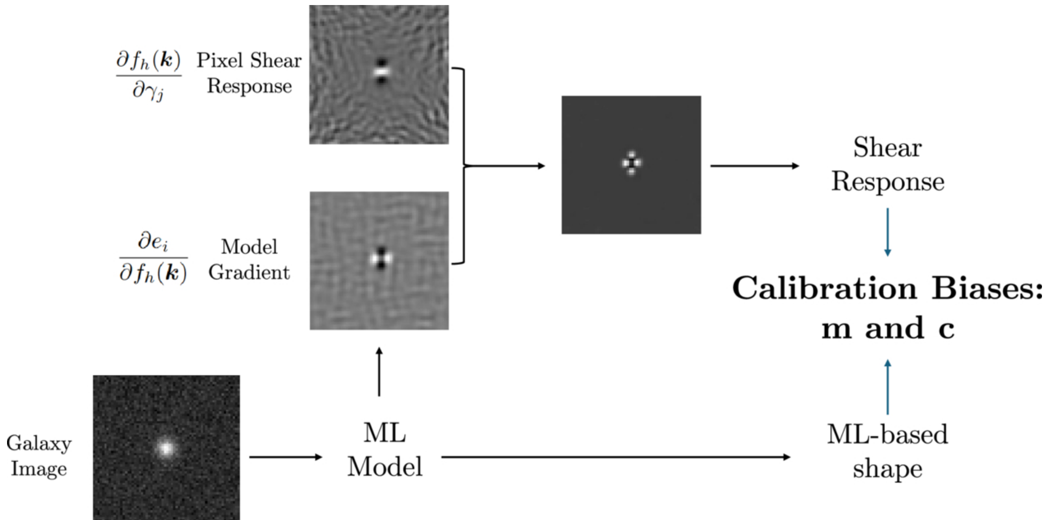
Figure 1. from Shurui Lin et al 2026 Astrophys. J. 1006 doi:10.3847/1538-4357/ae84b2 https://dx.doi.org/10.3847/1538-4357/ae84b2 © 2026. The Author(s). Published by the American Astronomical Society.
