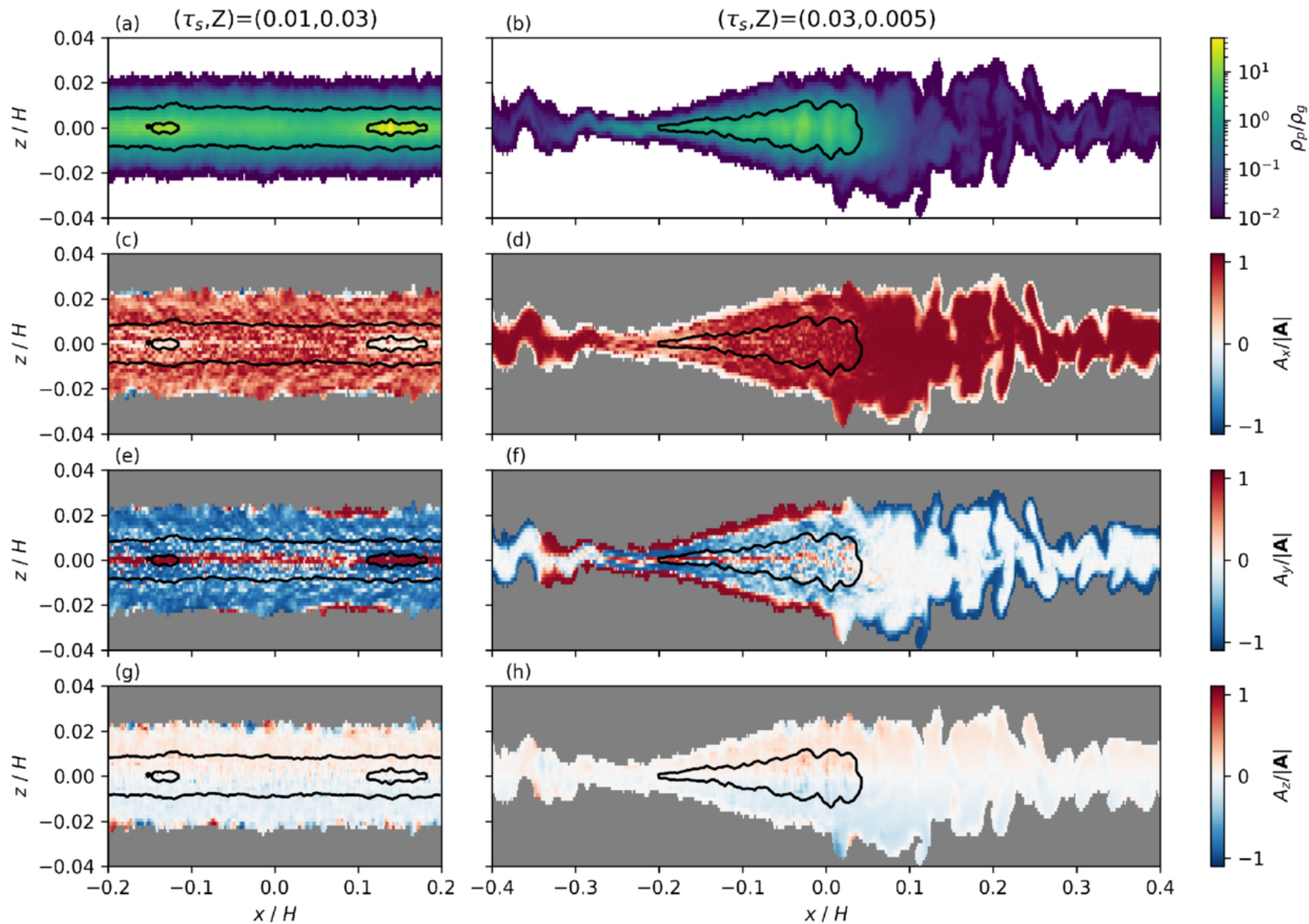
Figure 6. from Zhe-Yu Daniel Lin et al 2026 Astrophys. J. 1006 doi:10.3847/1538-4357/ae8445 https://dx.doi.org/10.3847/1538-4357/ae8445 © 2026. The Author(s). Published by the American Astronomical Society.
