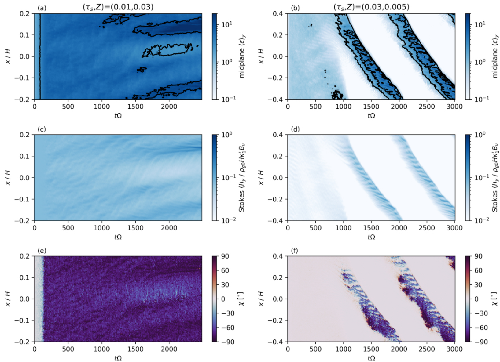
Figure 3. from Zhe-Yu Daniel Lin et al 2026 Astrophys. J. 1006 doi:10.3847/1538-4357/ae8445 https://dx.doi.org/10.3847/1538-4357/ae8445 © 2026. The Author(s). Published by the American Astronomical Society.
