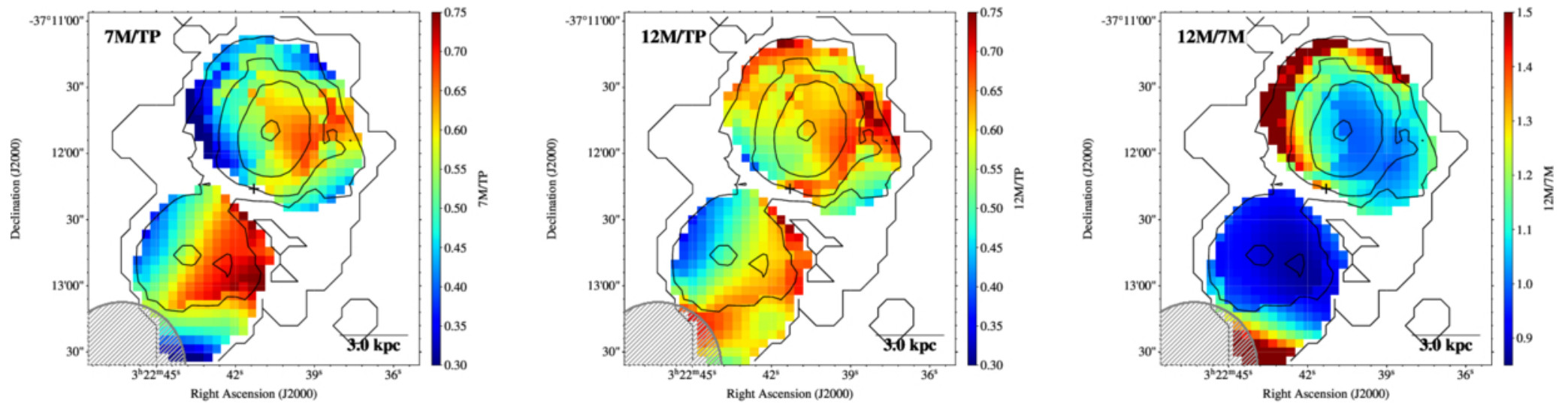
Figure 7. from Kana Morokuma-Matsui et al 2026 Astrophys. J. 1007 doi:10.3847/1538-4357/ae83a9 https://dx.doi.org/10.3847/1538-4357/ae83a9 © 2026. The Author(s). Published by the American Astronomical Society.
