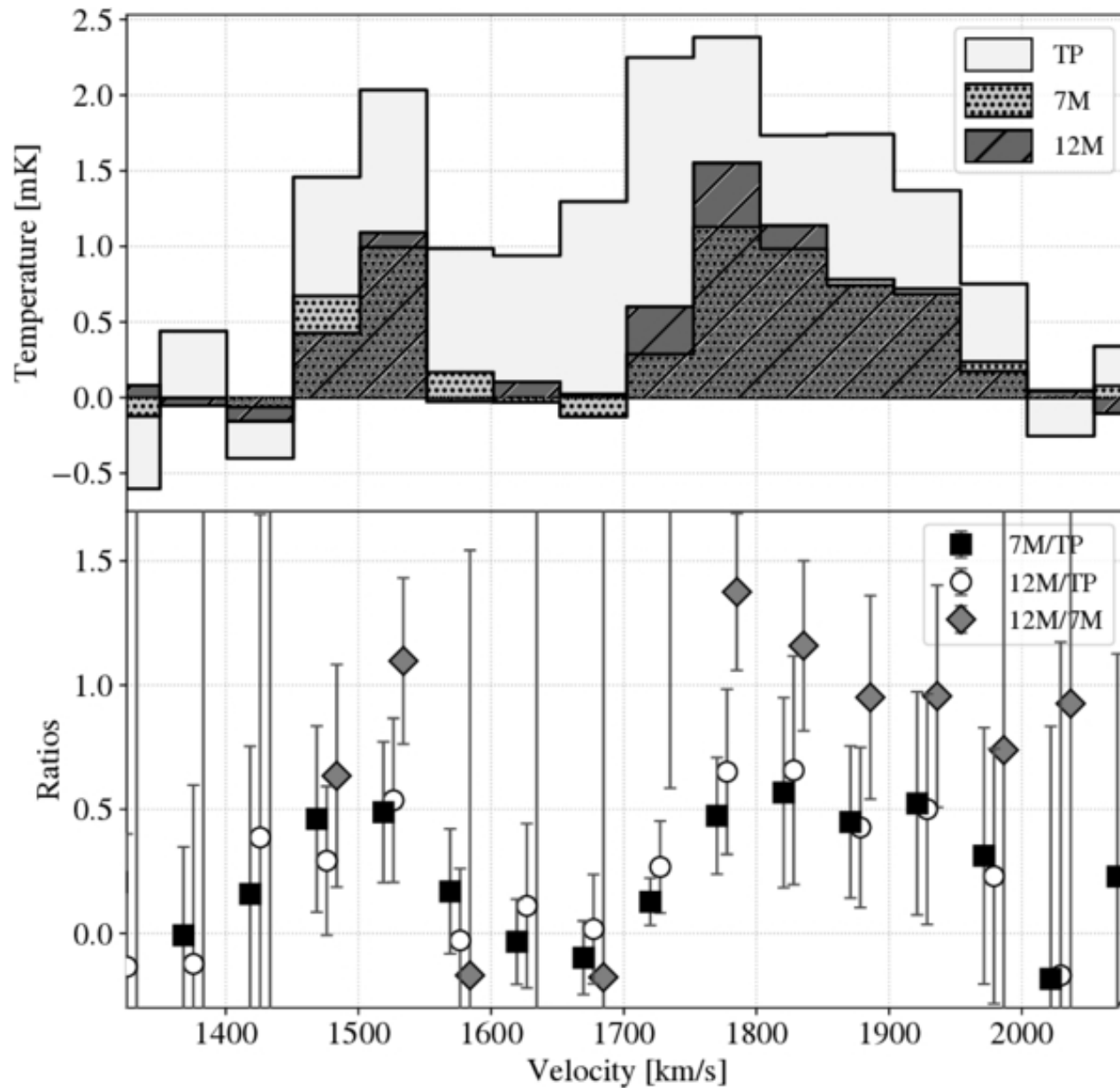
Figure 6. from Kana Morokuma-Matsui et al 2026 Astrophys. J. 1007 doi:10.3847/1538-4357/ae83a9 https://dx.doi.org/10.3847/1538-4357/ae83a9 © 2026. The Author(s). Published by the American Astronomical Society.
