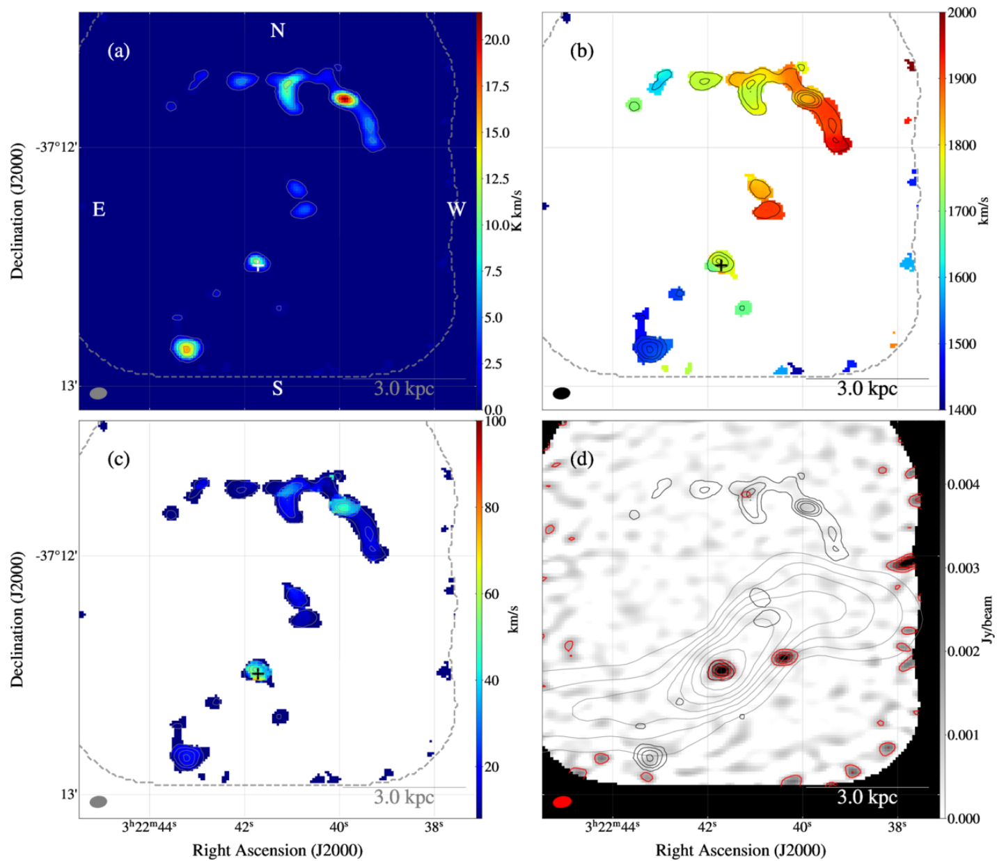
Figure 5. from Kana Morokuma-Matsui et al 2026 Astrophys. J. 1007 doi:10.3847/1538-4357/ae83a9 https://dx.doi.org/10.3847/1538-4357/ae83a9 © 2026. The Author(s). Published by the American Astronomical Society.
