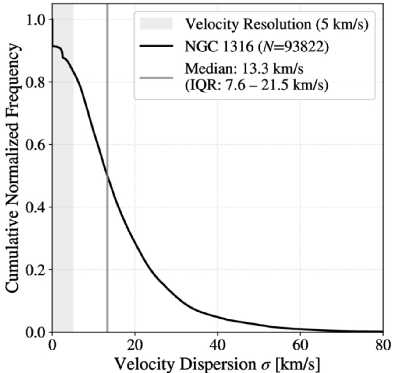
Figure 3. from Kana Morokuma-Matsui et al 2026 Astrophys. J. 1007 doi:10.3847/1538-4357/ae83a9 https://dx.doi.org/10.3847/1538-4357/ae83a9 © 2026. The Author(s). Published by the American Astronomical Society.
