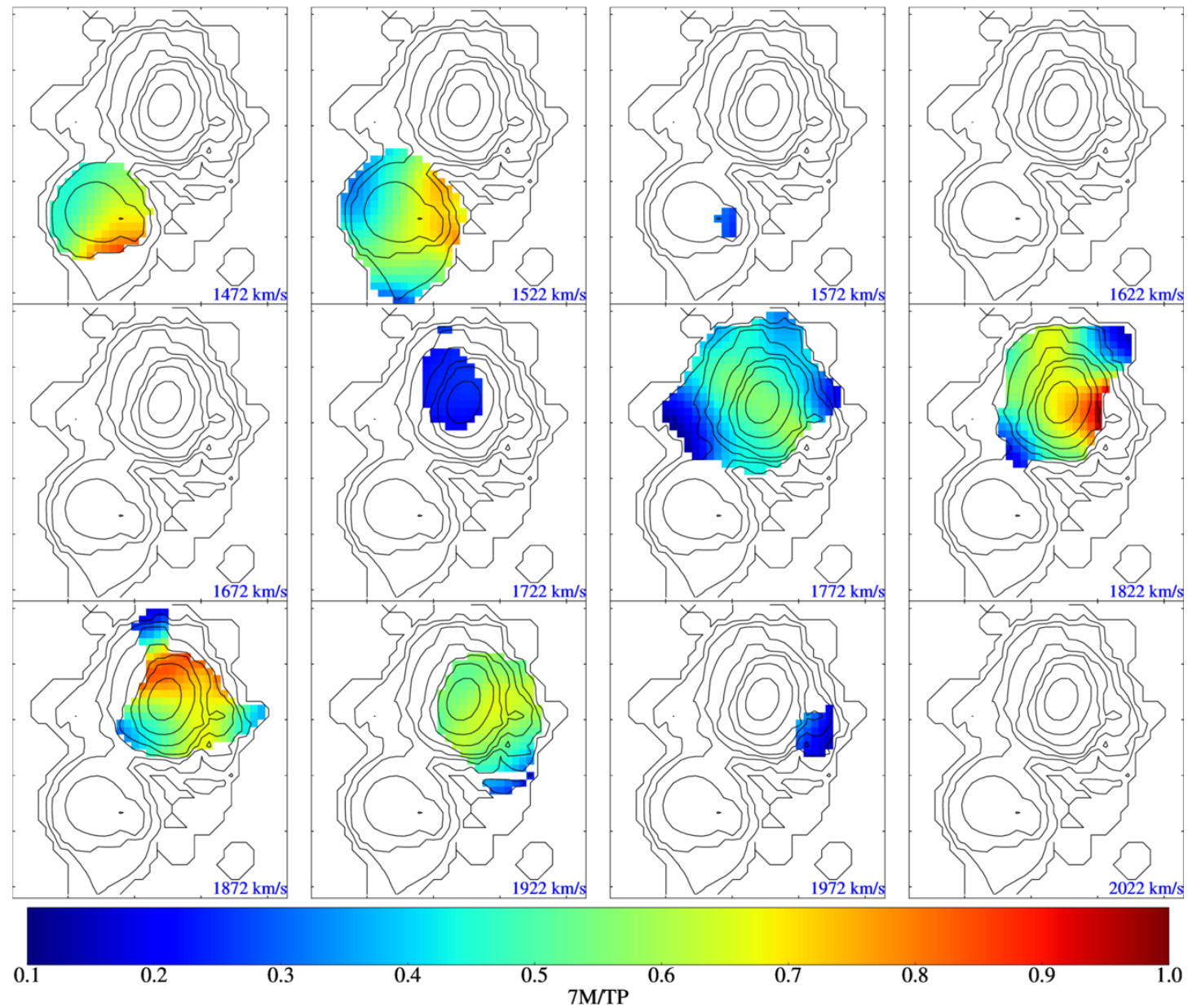
Figure 20. from Kana Morokuma-Matsui et al 2026 Astrophys. J. 1007 doi:10.3847/1538-4357/ae83a9 https://dx.doi.org/10.3847/1538-4357/ae83a9 © 2026. The Author(s). Published by the American Astronomical Society.
