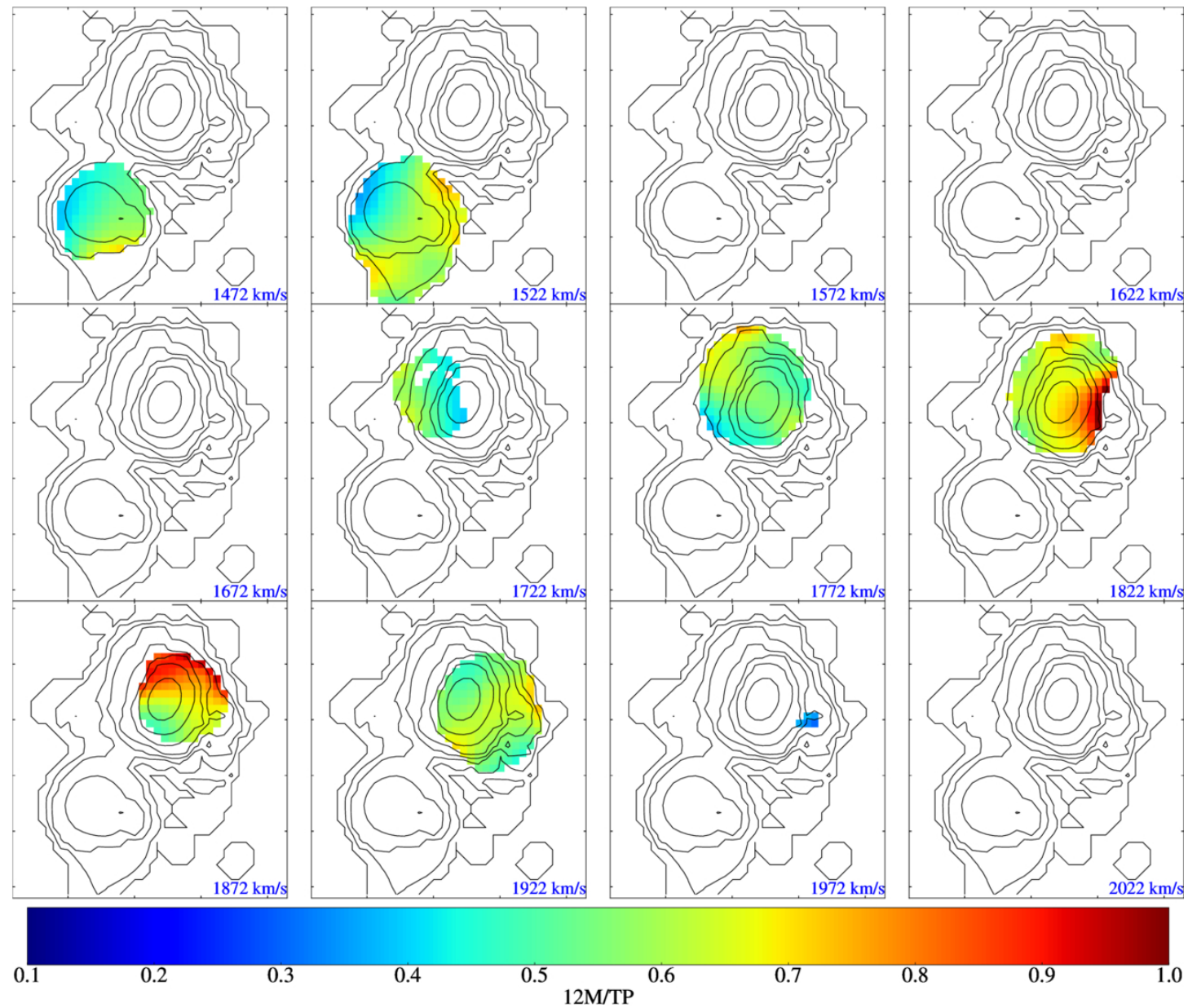
Figure 19. from Kana Morokuma-Matsui et al 2026 Astrophys. J. 1007 doi:10.3847/1538-4357/ae83a9 https://dx.doi.org/10.3847/1538-4357/ae83a9 © 2026. The Author(s). Published by the American Astronomical Society.
