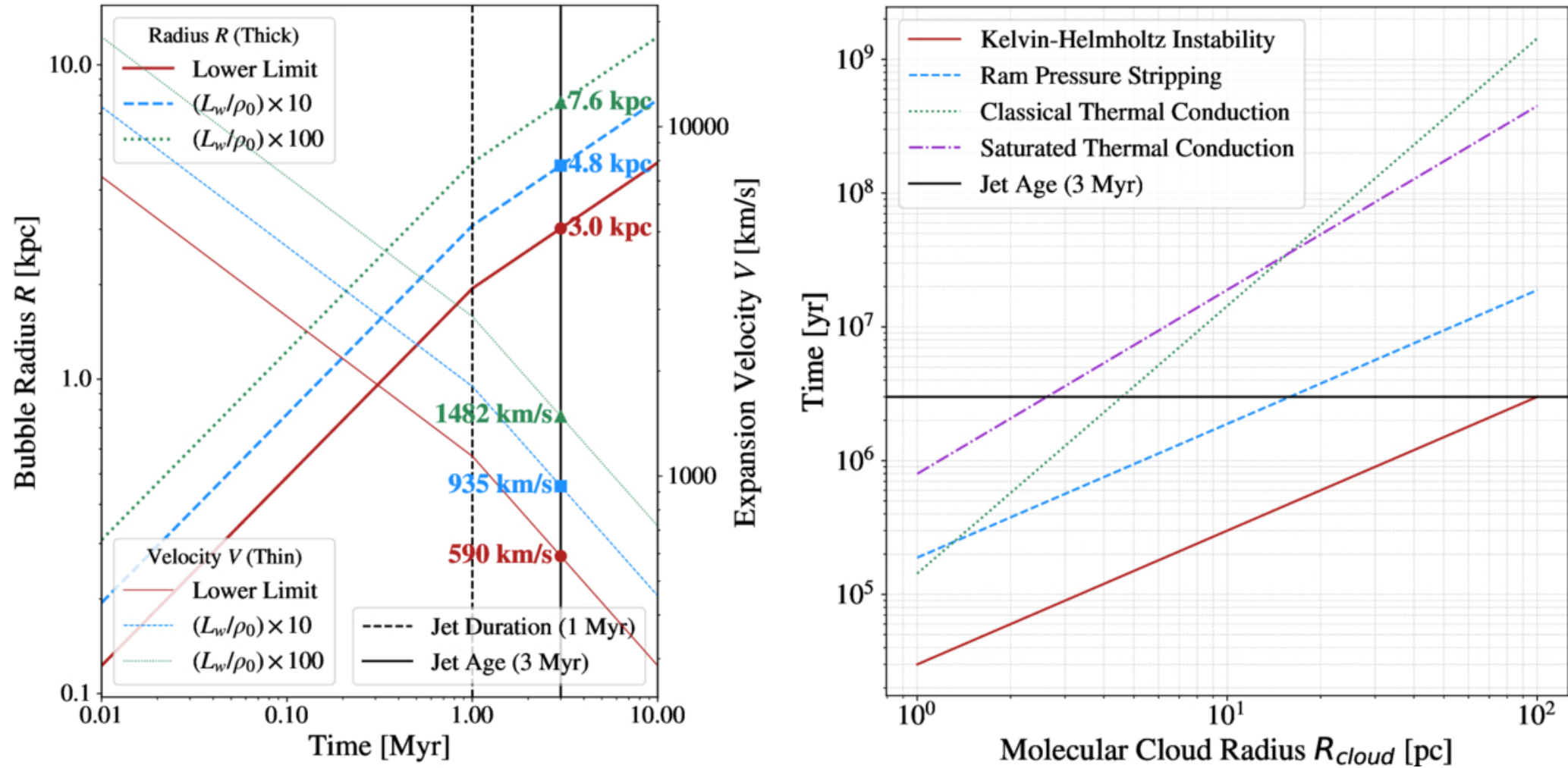
Figure 18. from Kana Morokuma-Matsui et al 2026 Astrophys. J. 1007 doi:10.3847/1538-4357/ae83a9 https://dx.doi.org/10.3847/1538-4357/ae83a9 © 2026. The Author(s). Published by the American Astronomical Society.
