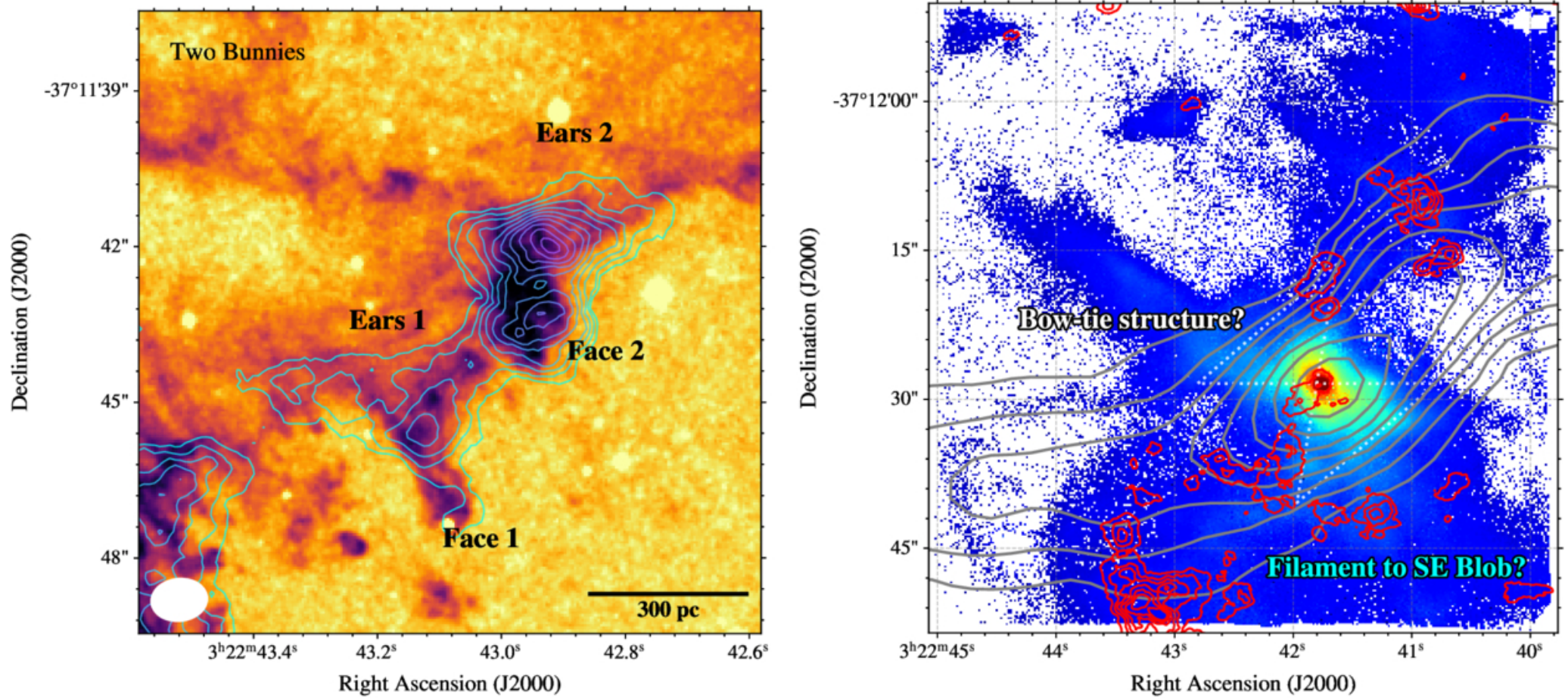
Figure 17. from Kana Morokuma-Matsui et al 2026 Astrophys. J. 1007 doi:10.3847/1538-4357/ae83a9 https://dx.doi.org/10.3847/1538-4357/ae83a9 © 2026. The Author(s). Published by the American Astronomical Society.
