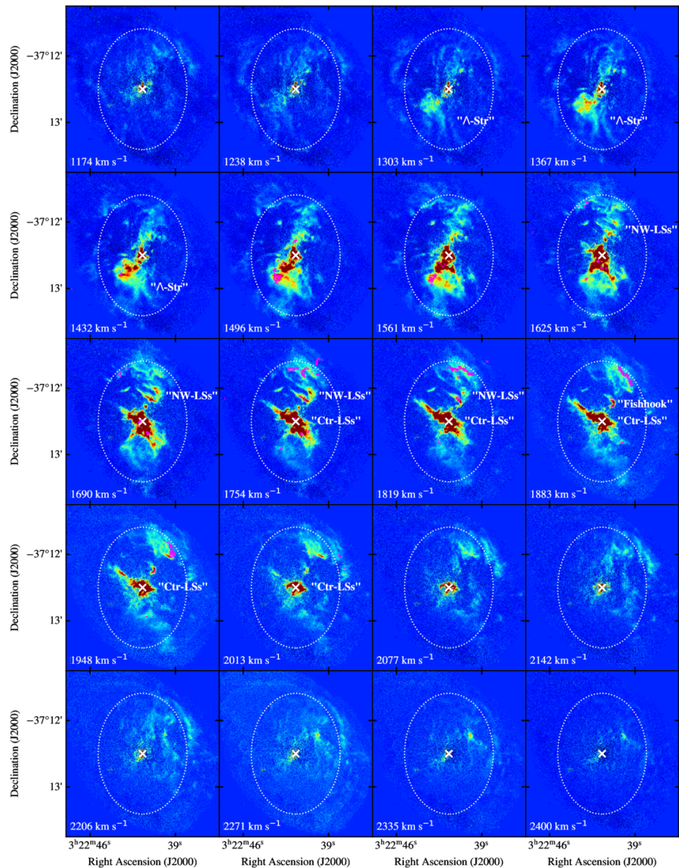
Figure 16. from Kana Morokuma-Matsui et al 2026 Astrophys. J. 1007 doi:10.3847/1538-4357/ae83a9 https://dx.doi.org/10.3847/1538-4357/ae83a9 © 2026. The Author(s). Published by the American Astronomical Society.
