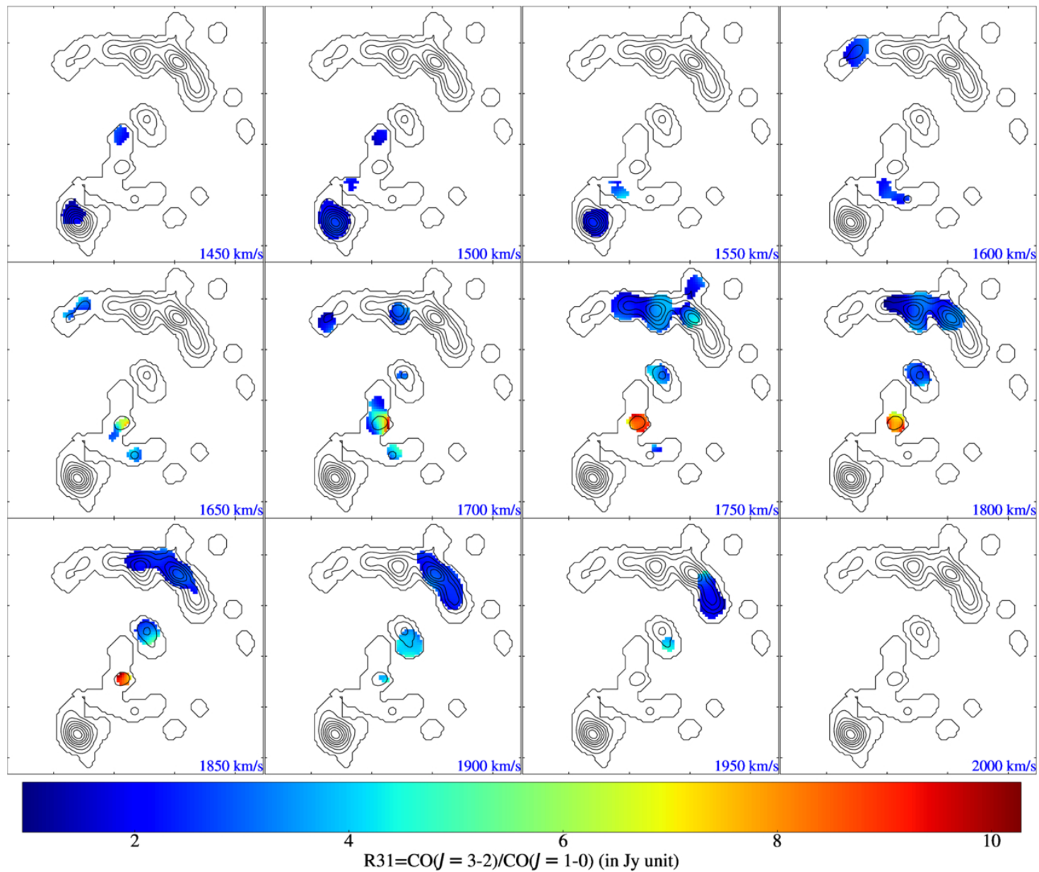
Figure 14. from Kana Morokuma-Matsui et al 2026 Astrophys. J. 1007 doi:10.3847/1538-4357/ae83a9 https://dx.doi.org/10.3847/1538-4357/ae83a9 © 2026. The Author(s). Published by the American Astronomical Society.
