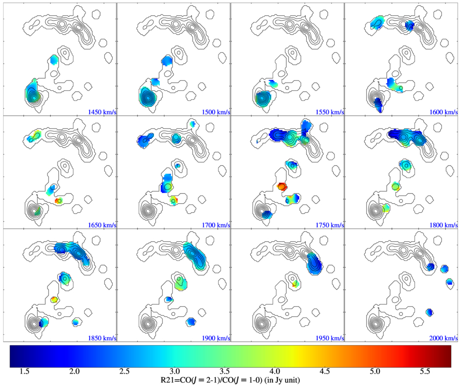
Figure 13. from Kana Morokuma-Matsui et al 2026 Astrophys. J. 1007 doi:10.3847/1538-4357/ae83a9 https://dx.doi.org/10.3847/1538-4357/ae83a9 © 2026. The Author(s). Published by the American Astronomical Society.
