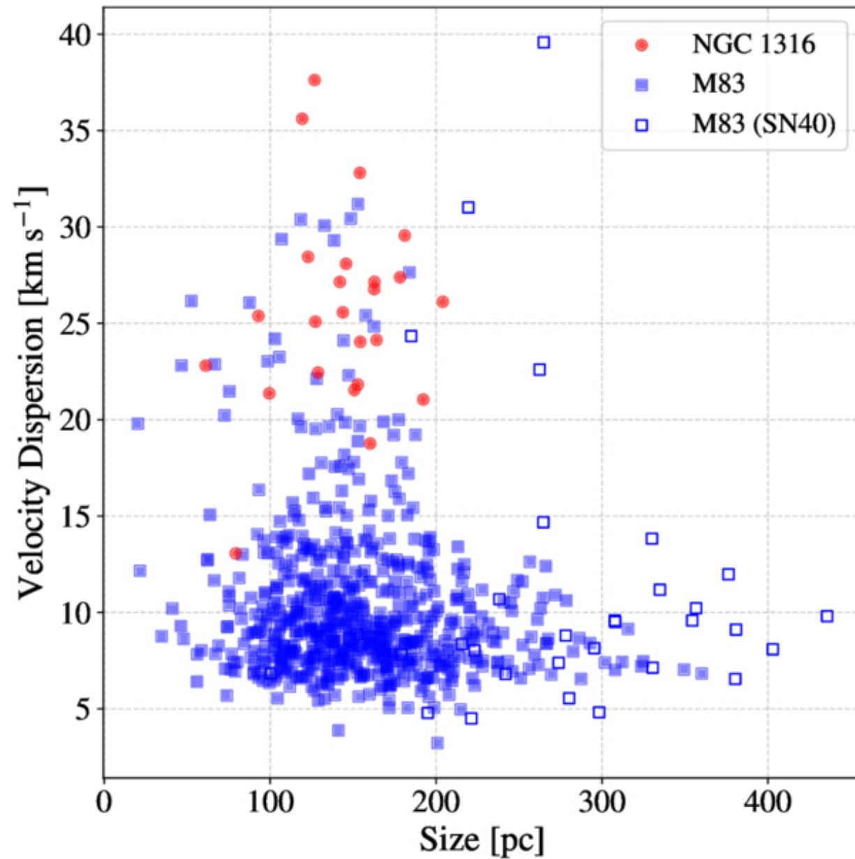
Figure 10. from Kana Morokuma-Matsui et al 2026 Astrophys. J. 1007 doi:10.3847/1538-4357/ae83a9 https://dx.doi.org/10.3847/1538-4357/ae83a9 © 2026. The Author(s). Published by the American Astronomical Society.
