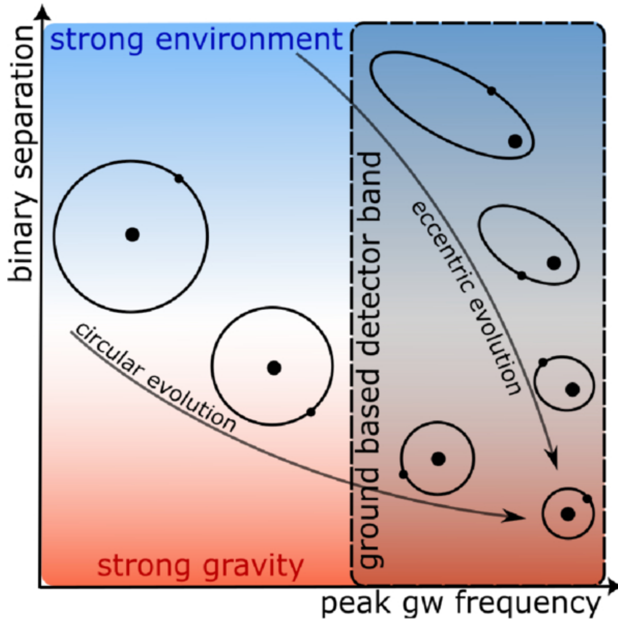
Figure 1. from Lorenz Zwick et al 2026 Astrophys. J. 1006 doi:10.3847/1538-4357/ae839d https://dx.doi.org/10.3847/1538-4357/ae839d © 2026. The Author(s). Published by the American Astronomical Society.
