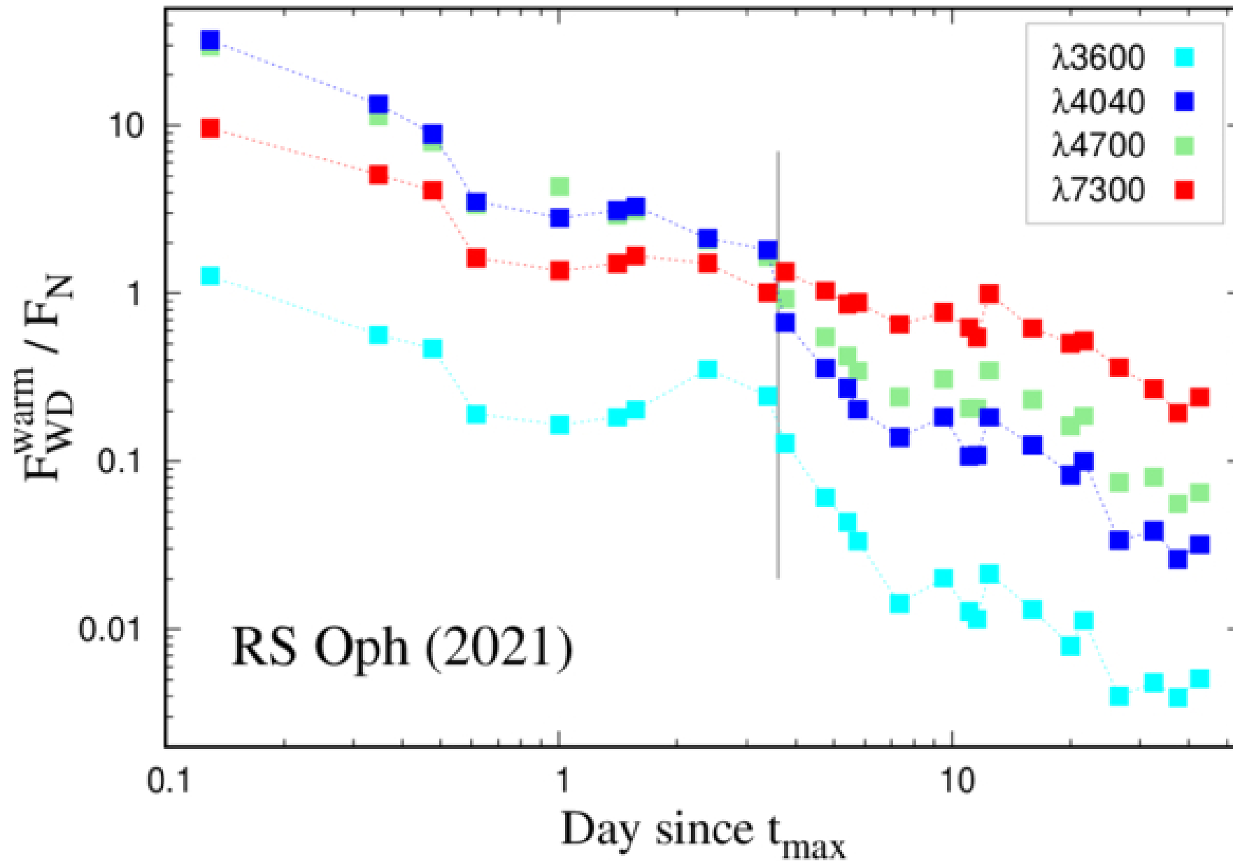
Figure 9. from Augustin Skopal et al 2026 Astrophys. J. 1007 doi:10.3847/1538-4357/ae82d5 https://dx.doi.org/10.3847/1538-4357/ae82d5 © 2026. The Author(s). Published by the American Astronomical Society.
