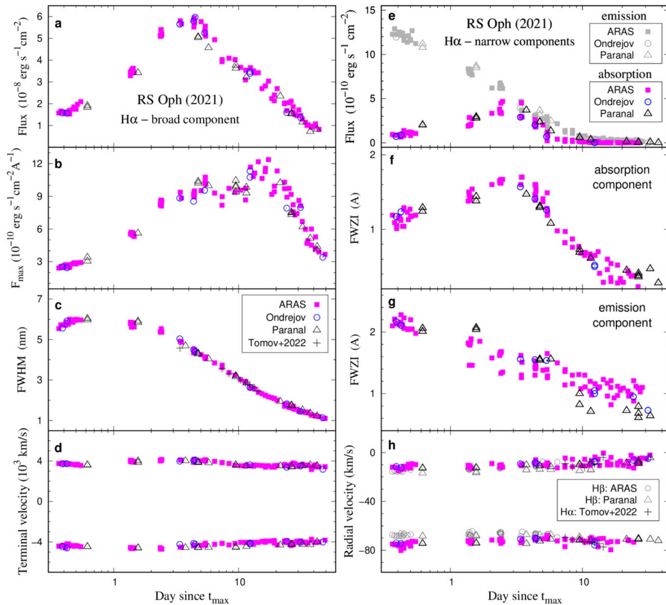
Figure 8. from Augustin Skopal et al 2026 Astrophys. J. 1007 doi:10.3847/1538-4357/ae82d5 https://dx.doi.org/10.3847/1538-4357/ae82d5 © 2026. The Author(s). Published by the American Astronomical Society.
