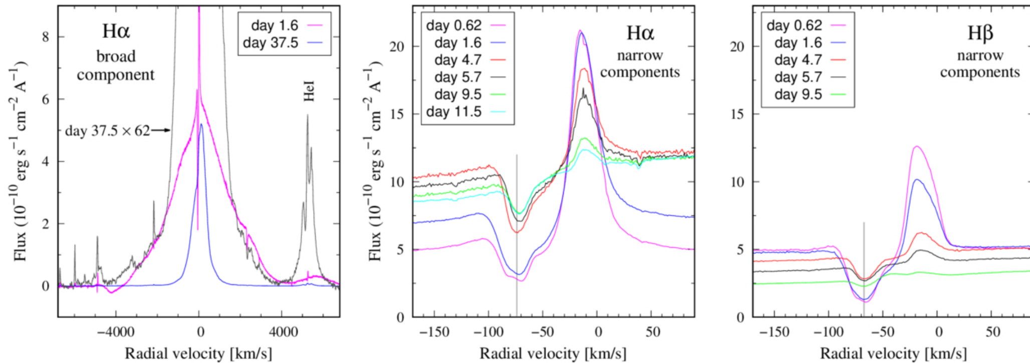
Figure 7. from Augustin Skopal et al 2026 Astrophys. J. 1007 doi:10.3847/1538-4357/ae82d5 https://dx.doi.org/10.3847/1538-4357/ae82d5 © 2026. The Author(s). Published by the American Astronomical Society.
