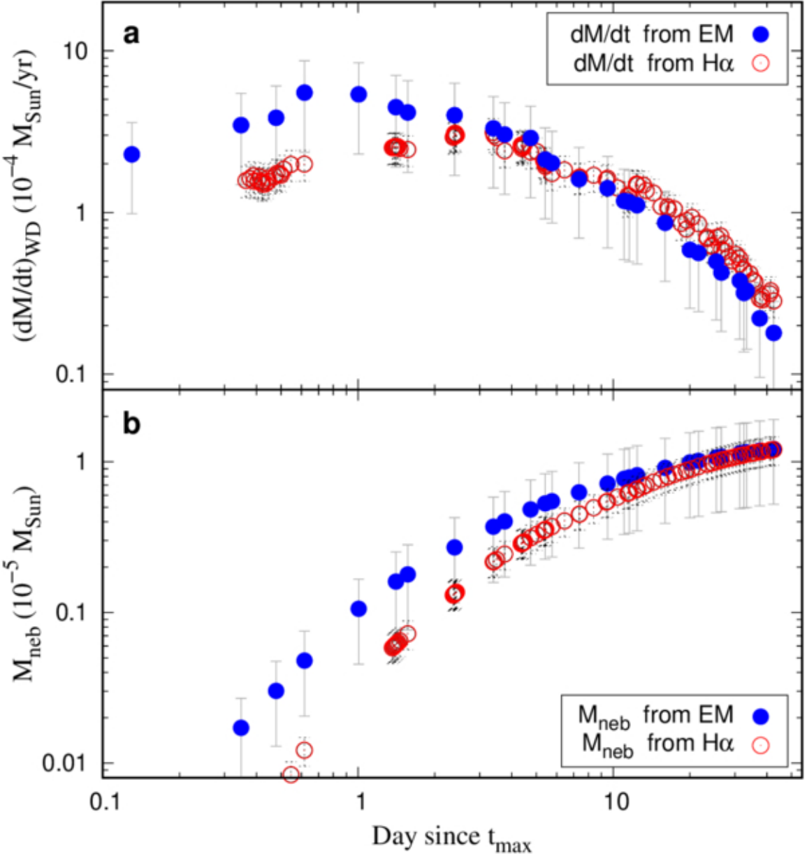
Figure 6. from Augustin Skopal et al 2026 Astrophys. J. 1007 doi:10.3847/1538-4357/ae82d5 https://dx.doi.org/10.3847/1538-4357/ae82d5 © 2026. The Author(s). Published by the American Astronomical Society.
