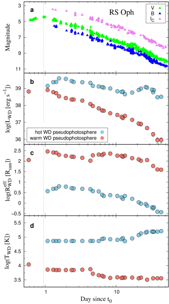
Figure 5. from Augustin Skopal et al 2026 Astrophys. J. 1007 doi:10.3847/1538-4357/ae82d5 https://dx.doi.org/10.3847/1538-4357/ae82d5 © 2026. The Author(s). Published by the American Astronomical Society.
