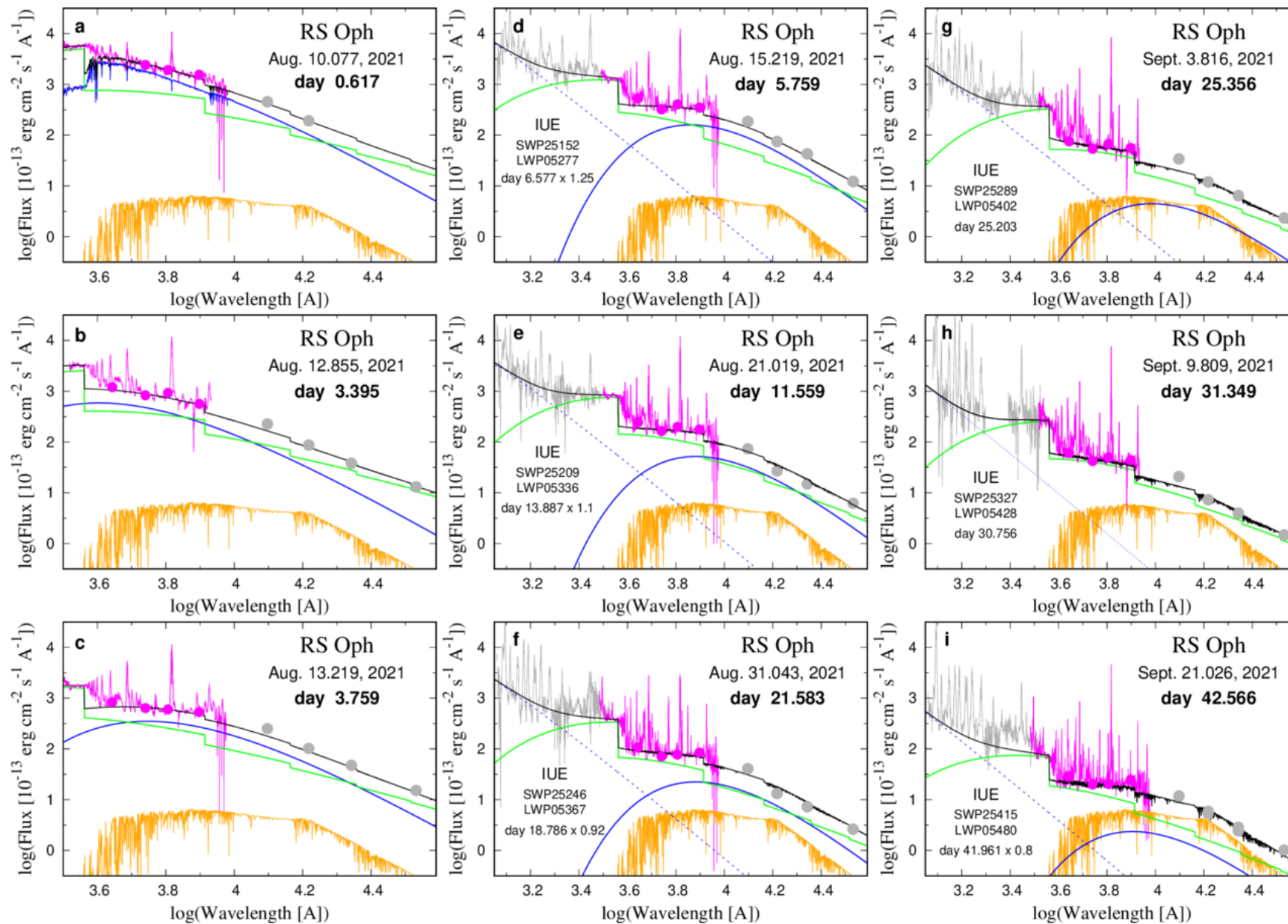
Figure 4. from Augustin Skopal et al 2026 Astrophys. J. 1007 doi:10.3847/1538-4357/ae82d5 https://dx.doi.org/10.3847/1538-4357/ae82d5 © 2026. The Author(s). Published by the American Astronomical Society.
