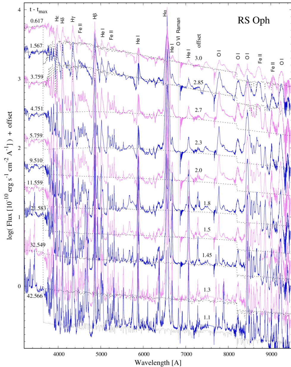
Figure 12. from Augustin Skopal et al 2026 Astrophys. J. 1007 doi:10.3847/1538-4357/ae82d5 https://dx.doi.org/10.3847/1538-4357/ae82d5 © 2026. The Author(s). Published by the American Astronomical Society.
