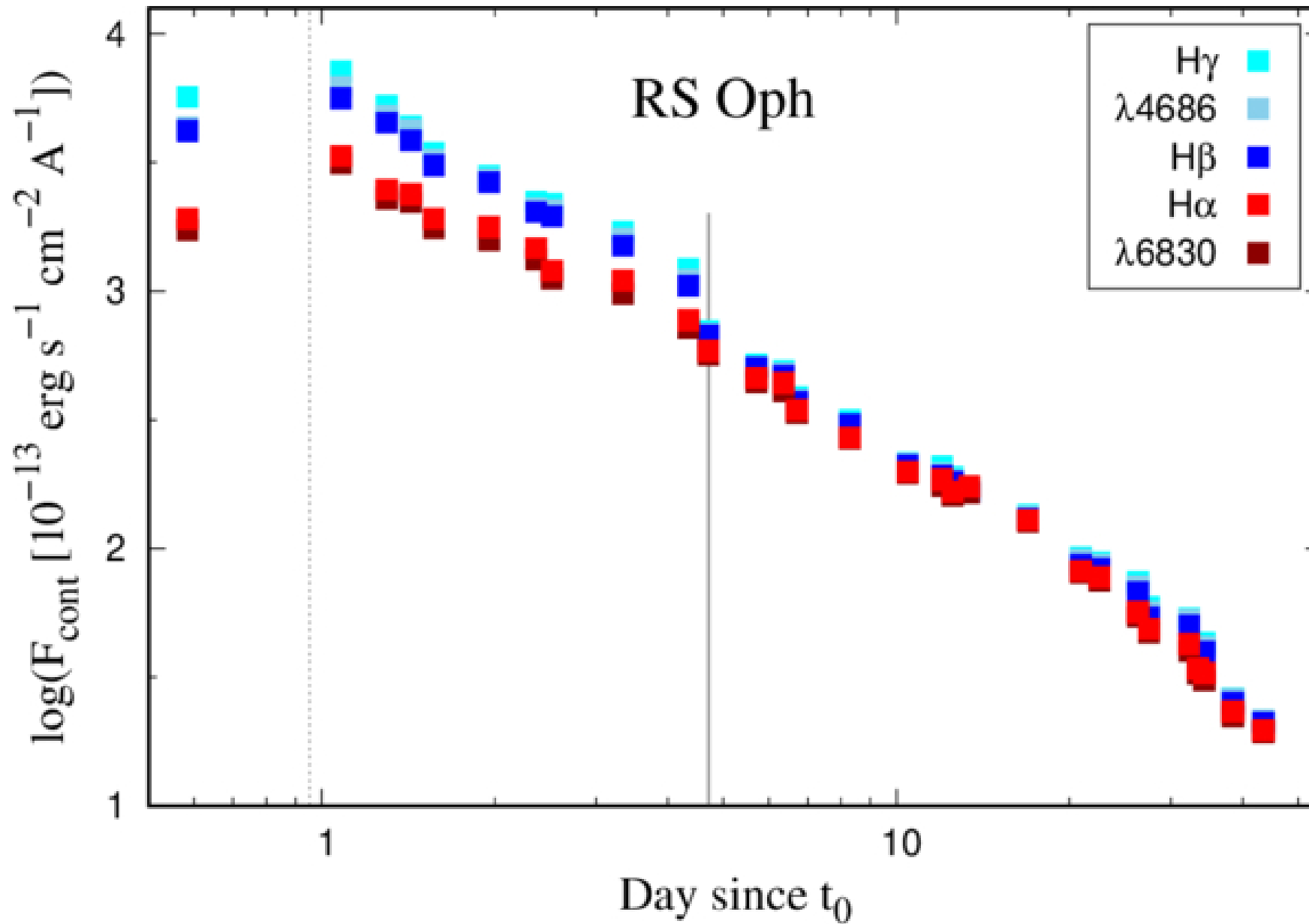
Figure 11. from Augustin Skopal et al 2026 Astrophys. J. 1007 doi:10.3847/1538-4357/ae82d5 https://dx.doi.org/10.3847/1538-4357/ae82d5 © 2026. The Author(s). Published by the American Astronomical Society.
