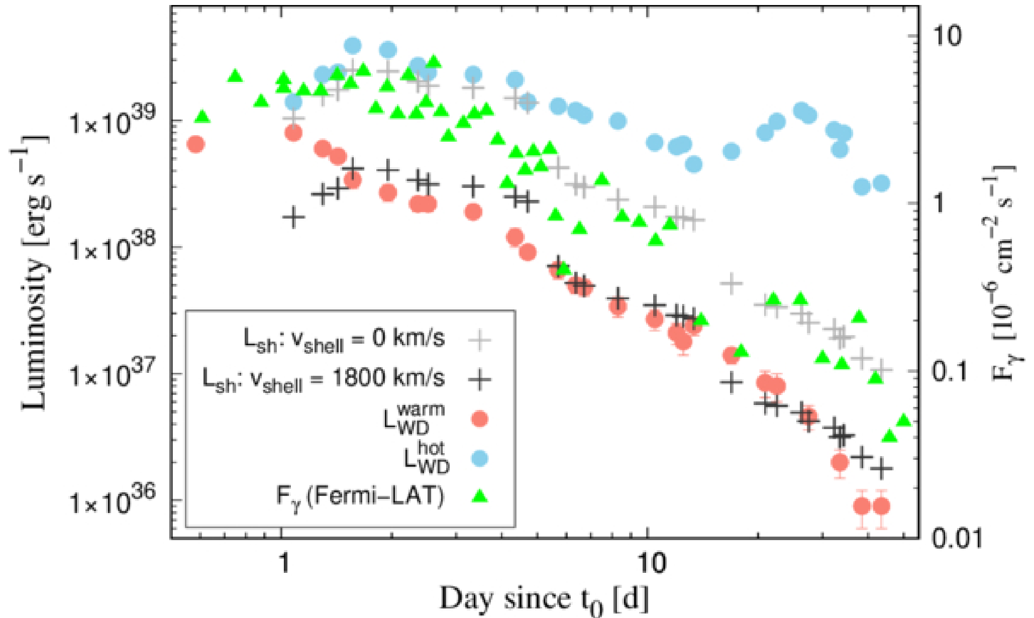
Figure 10. from Augustin Skopal et al 2026 Astrophys. J. 1007 doi:10.3847/1538-4357/ae82d5 https://dx.doi.org/10.3847/1538-4357/ae82d5 © 2026. The Author(s). Published by the American Astronomical Society.
