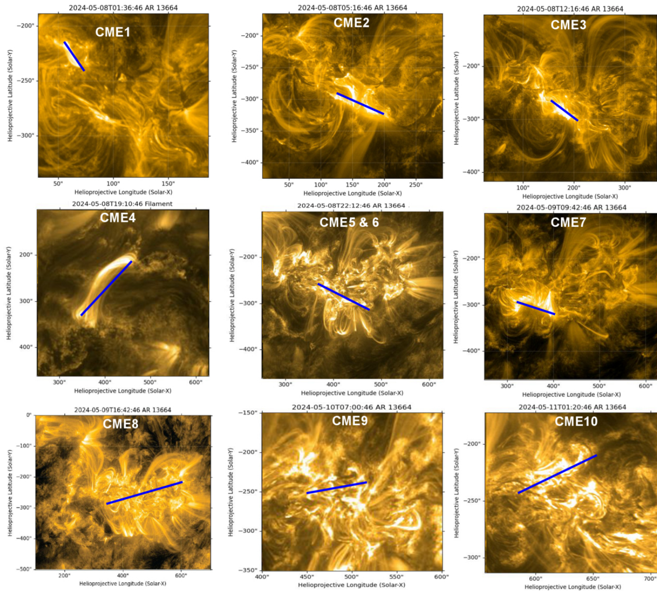
Figure A2. from Shirsh Lata Soni et al 2026 Astrophys. J. 1007 doi:10.3847/1538-4357/ae825e https://dx.doi.org/10.3847/1538-4357/ae825e © 2026. The Author(s). Published by the American Astronomical Society.
