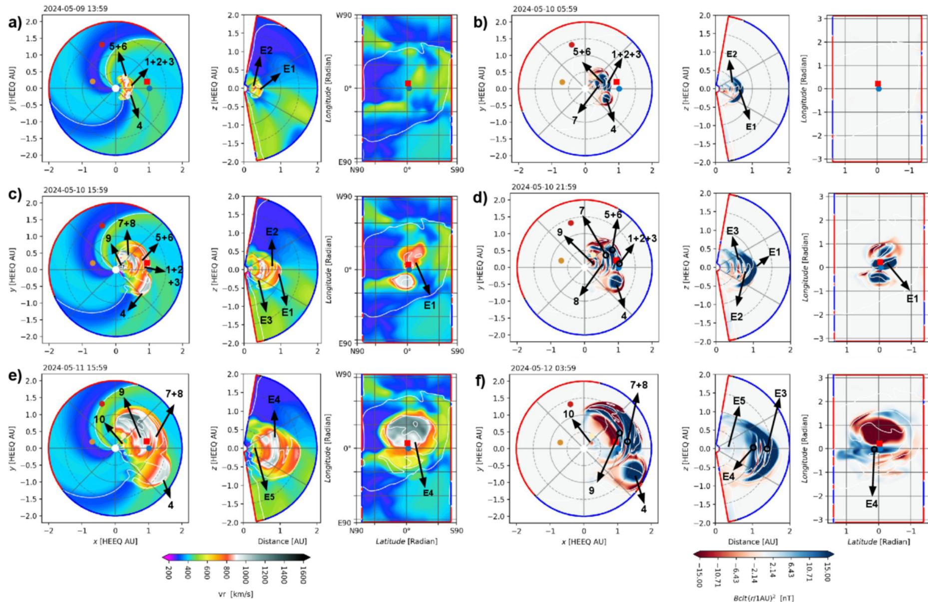
Figure 4. from Shirsh Lata Soni et al 2026 Astrophys. J. 1007 doi:10.3847/1538-4357/ae825e https://dx.doi.org/10.3847/1538-4357/ae825e © 2026. The Author(s). Published by the American Astronomical Society.
