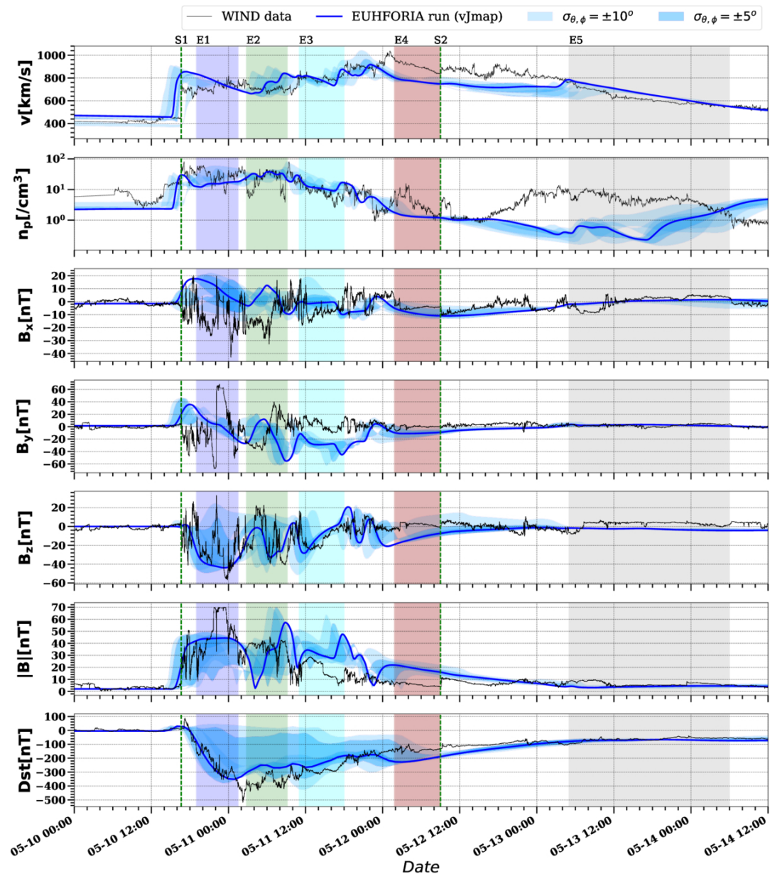
Figure 3. from Shirsh Lata Soni et al 2026 Astrophys. J. 1007 doi:10.3847/1538-4357/ae825e https://dx.doi.org/10.3847/1538-4357/ae825e © 2026. The Author(s). Published by the American Astronomical Society.
