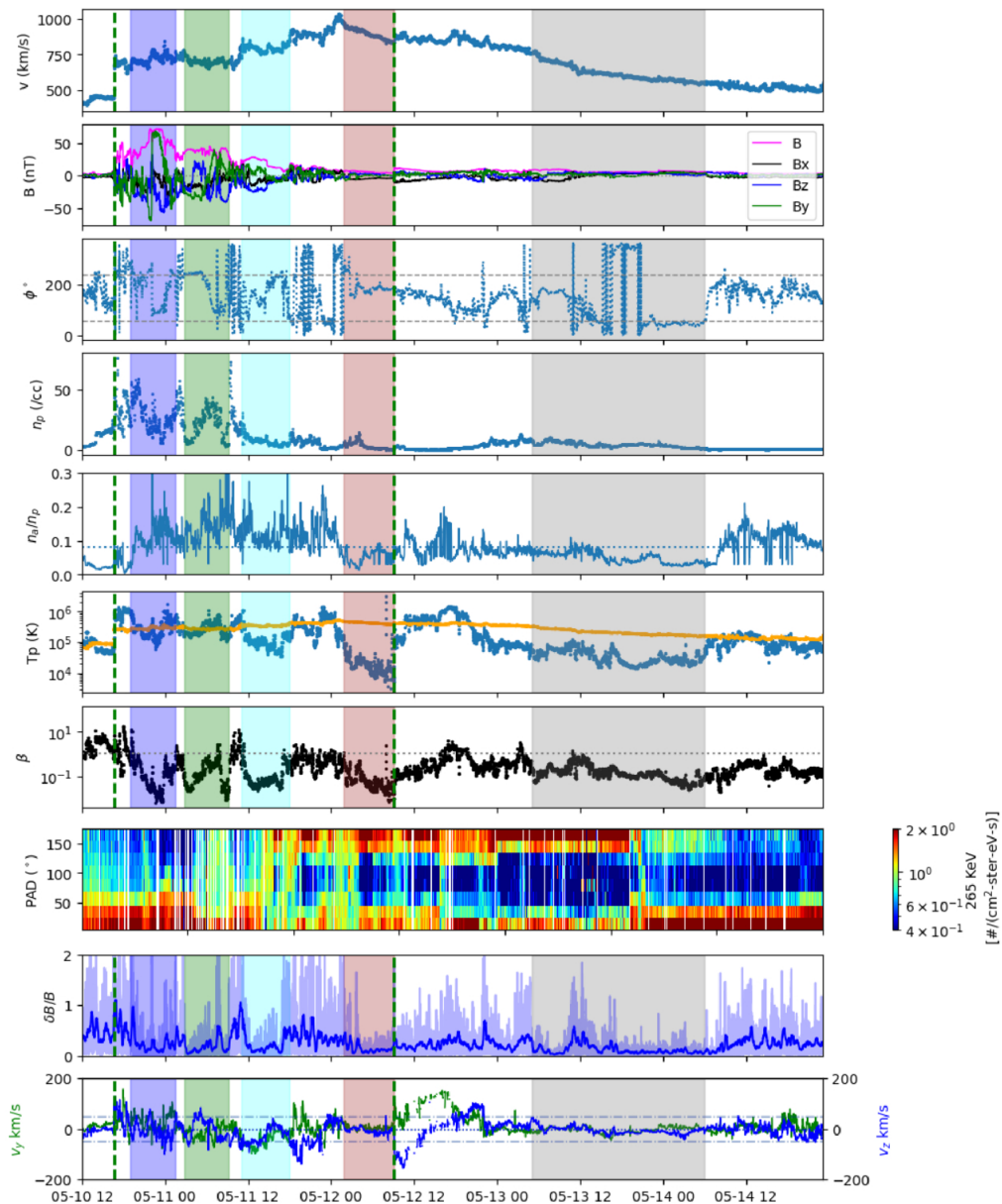
Figure 2. from Shirsh Lata Soni et al 2026 Astrophys. J. 1007 doi:10.3847/1538-4357/ae825e https://dx.doi.org/10.3847/1538-4357/ae825e © 2026. The Author(s). Published by the American Astronomical Society.
