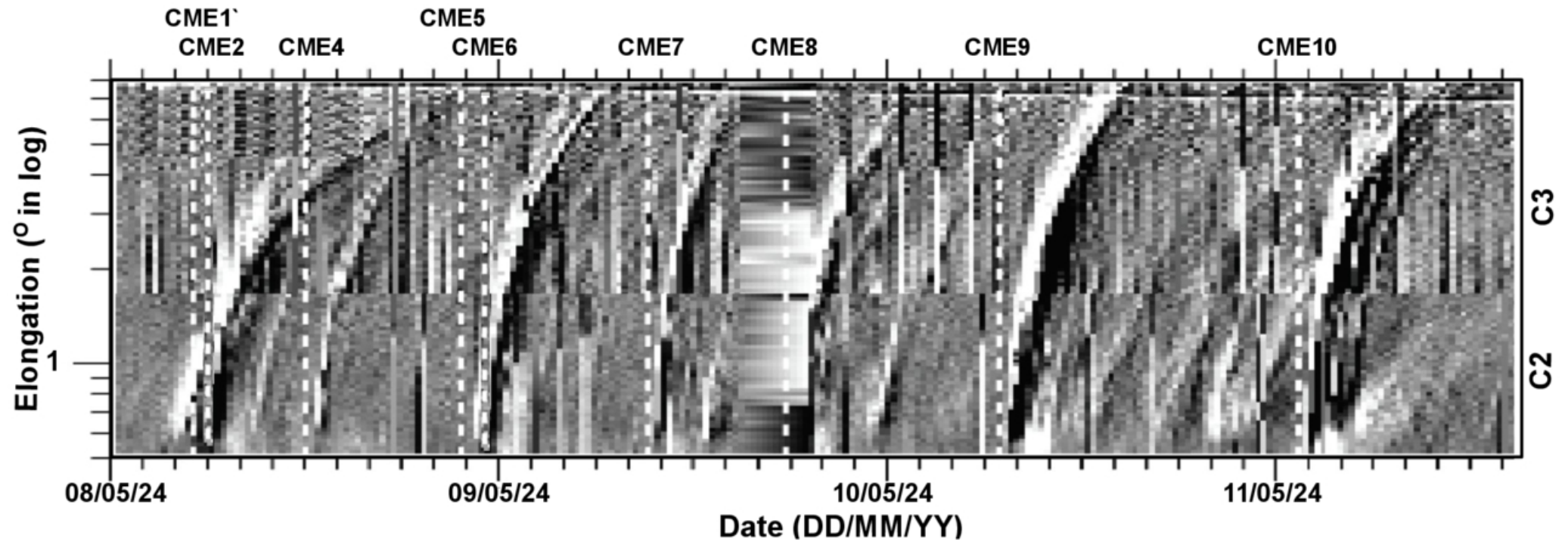
Figure 1. from Shirsh Lata Soni et al 2026 Astrophys. J. 1007 doi:10.3847/1538-4357/ae825e https://dx.doi.org/10.3847/1538-4357/ae825e © 2026. The Author(s). Published by the American Astronomical Society.
