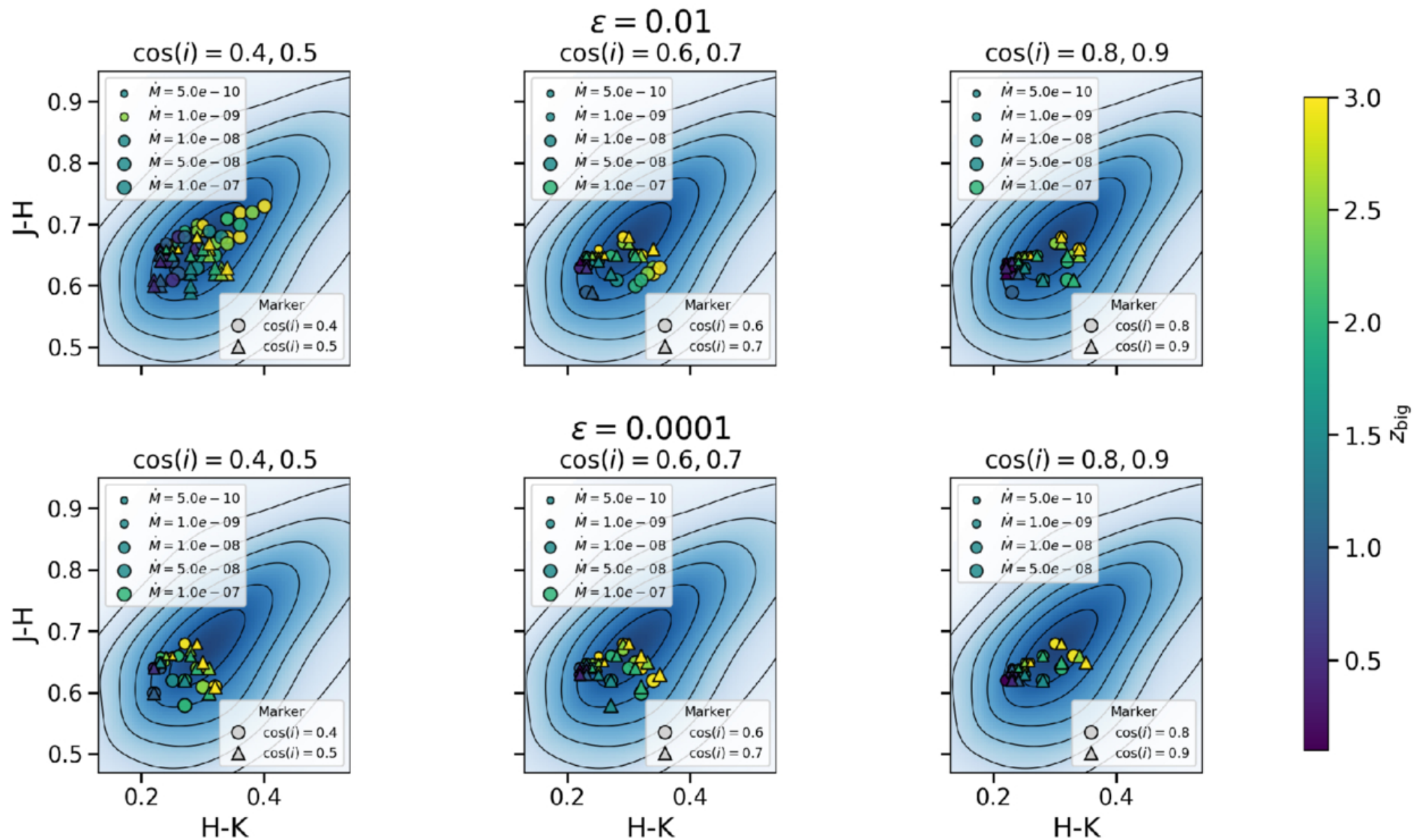
Figure 9. from Ezequiel Manzo-Martínez et al 2026 Astrophys. J. 1006 doi:10.3847/1538-4357/ae8255 https://dx.doi.org/10.3847/1538-4357/ae8255 © 2026. The Author(s). Published by the American Astronomical Society.
