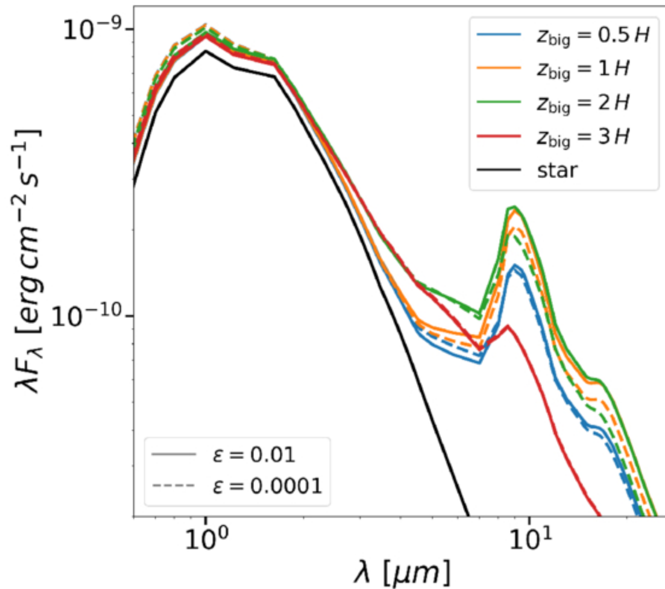
Figure 7. from Ezequiel Manzo-Martínez et al 2026 Astrophys. J. 1006 doi:10.3847/1538-4357/ae8255 https://dx.doi.org/10.3847/1538-4357/ae8255 © 2026. The Author(s). Published by the American Astronomical Society.
