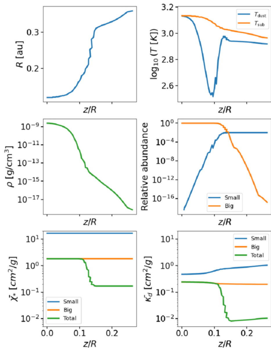
Figure 6. from Ezequiel Manzo-Martínez et al 2026 Astrophys. J. 1006 doi:10.3847/1538-4357/ae8255 https://dx.doi.org/10.3847/1538-4357/ae8255 © 2026. The Author(s). Published by the American Astronomical Society.
