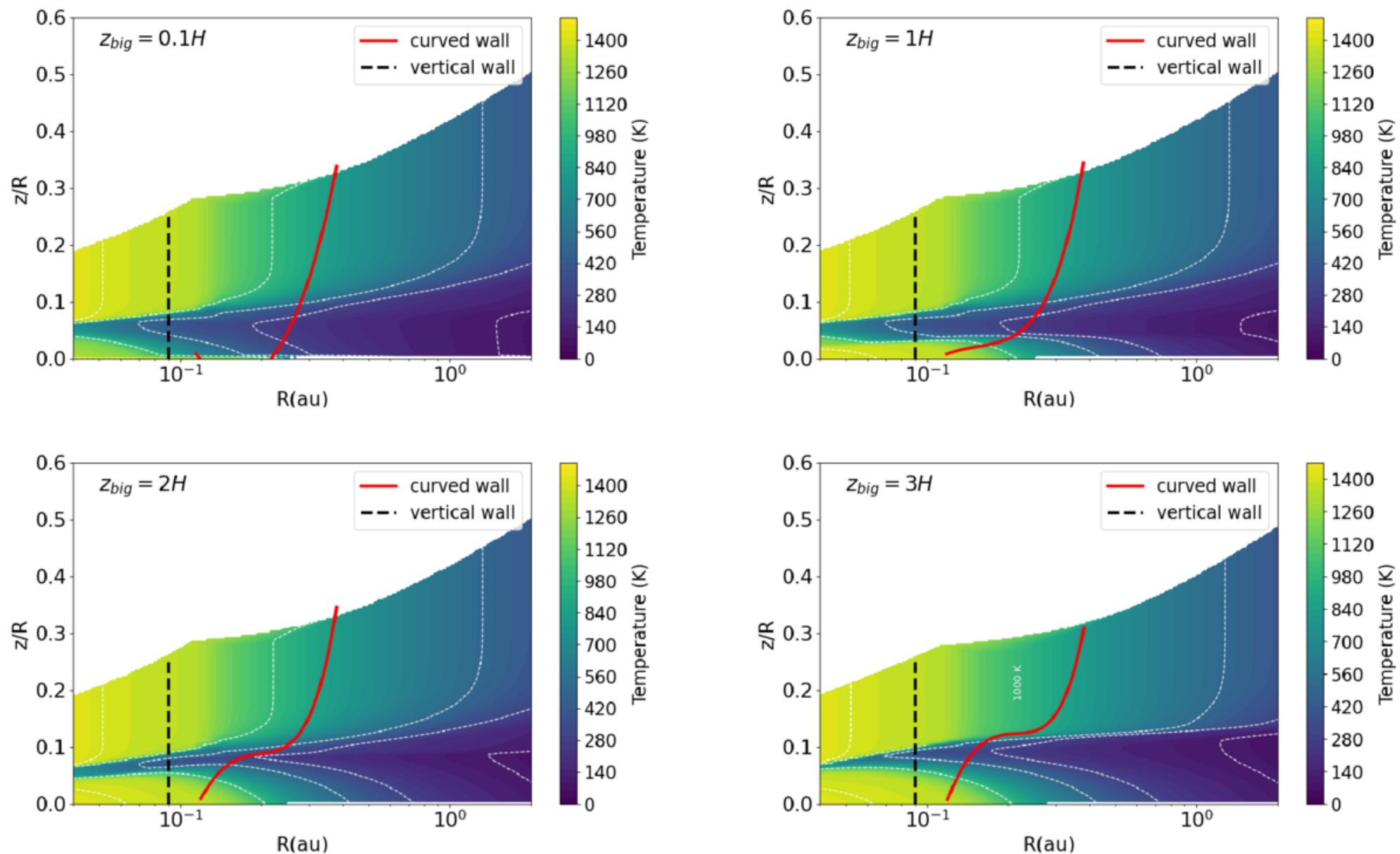
Figure 5. from Ezequiel Manzo-Martínez et al 2026 Astrophys. J. 1006 doi:10.3847/1538-4357/ae8255 https://dx.doi.org/10.3847/1538-4357/ae8255 © 2026. The Author(s). Published by the American Astronomical Society.
